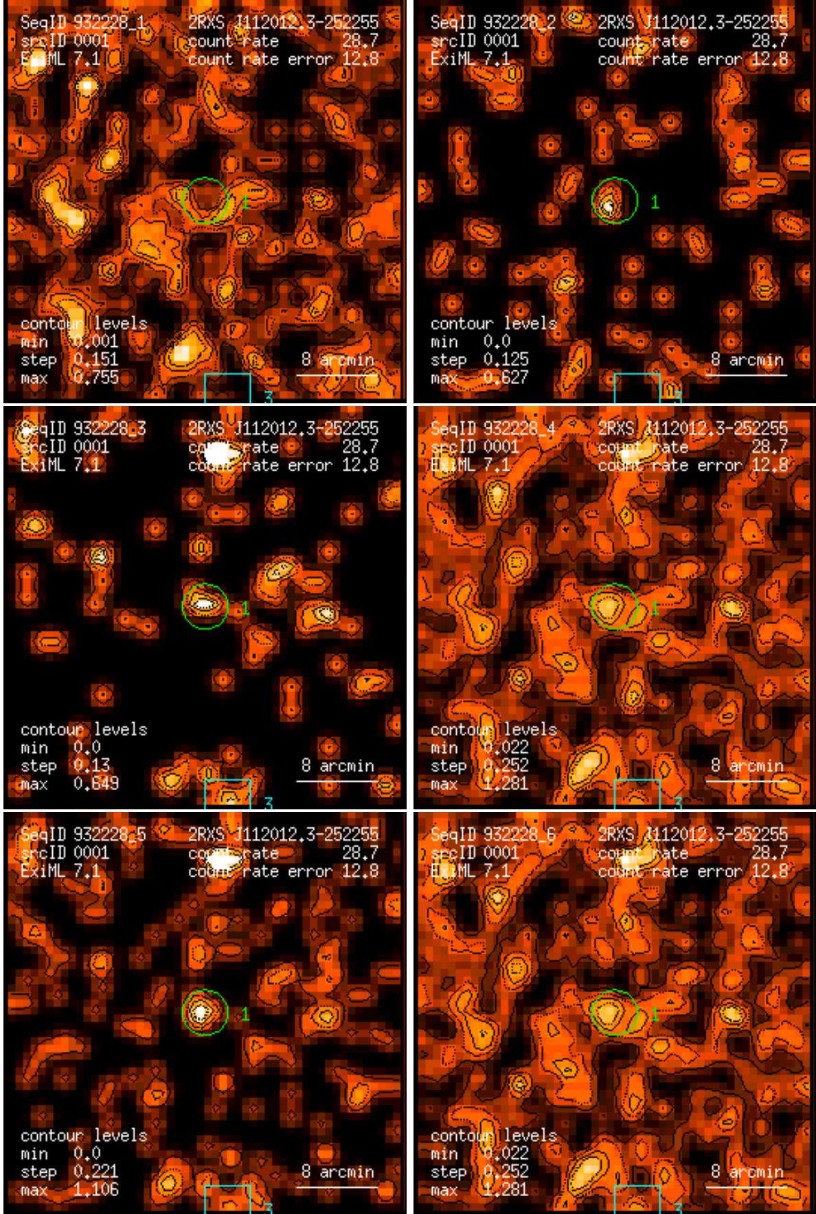
Figure 1: RASS 932228: detection 0001: band rate images, Gaussian filter: (1) PSPC channels 11 – 41, (2) 52 – 90, (3) 91 – 201, (4) 11 – 235, (5) 52 – 201, (6) 11 – 201. Broad band rates in counts/ks. Band rate contour levels in counts/ks/arcmin 2 .
