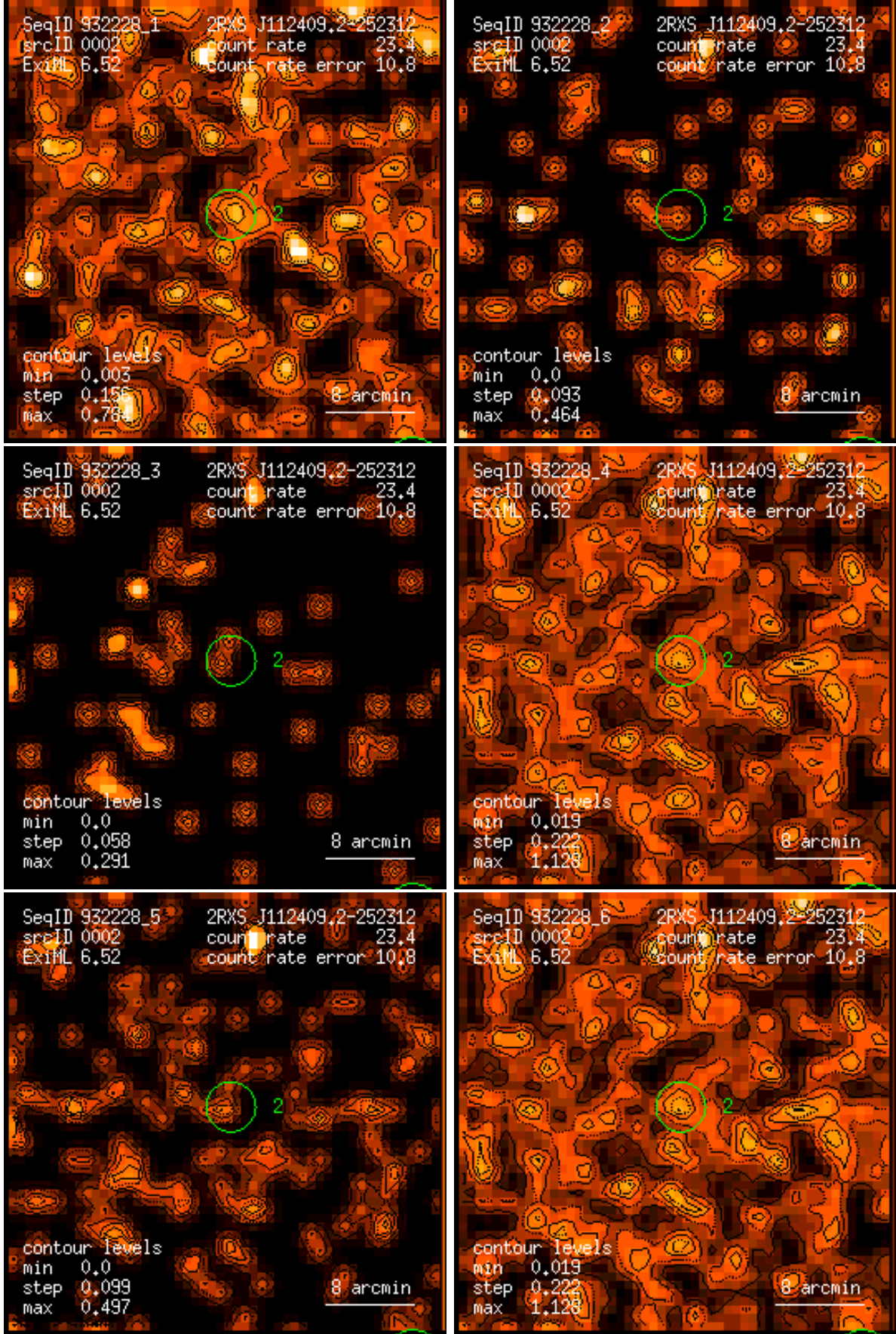
Figure 2: RASS 932228: detection 0002: band rate images, Gaussian filter: (1) PSPC channels 11 – 41, (2) 52 – 90, (3) 91 – 201, (4) 11 – 235, (5) 52 – 201, (6) 11 – 201. Broad band rates in counts/ks. Band rate contour levels in counts/ks/arcmin 2 .
