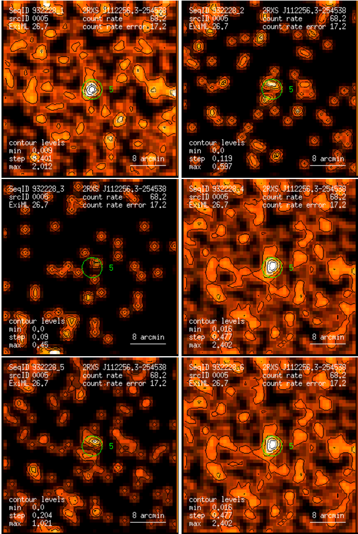
Figure 5: RASS 932228: detection 0005: band rate images, Gaussian filter: (1) PSPC channels 11 – 41, (2) 52 – 90, (3) 91 – 201, (4) 11 – 235, (5) 52 – 201, (6) 11 – 201. Broad band rates in counts/ks. Band rate contour levels in counts/ks/arcmin 2 .
