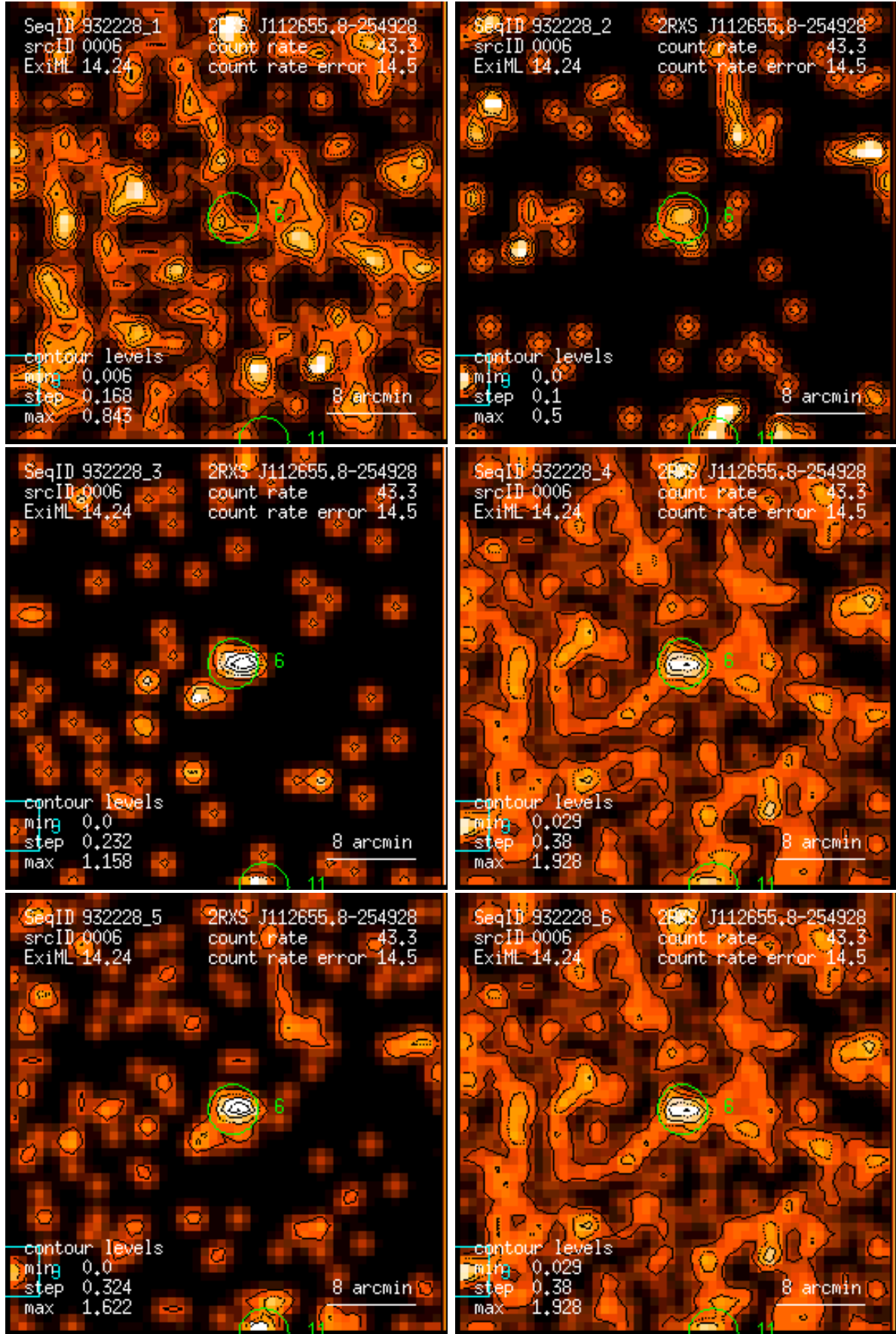
Figure 6: RASS 932228: detection 0006: band rate images, Gaussian filter: (1) PSPC channels 11 – 41, (2) 52 – 90, (3) 91 – 201, (4) 11 – 235, (5) 52 – 201, (6) 11 – 201. Broad band rates in counts/ks. Band rate contour levels in counts/ks/arcmin 2 .
