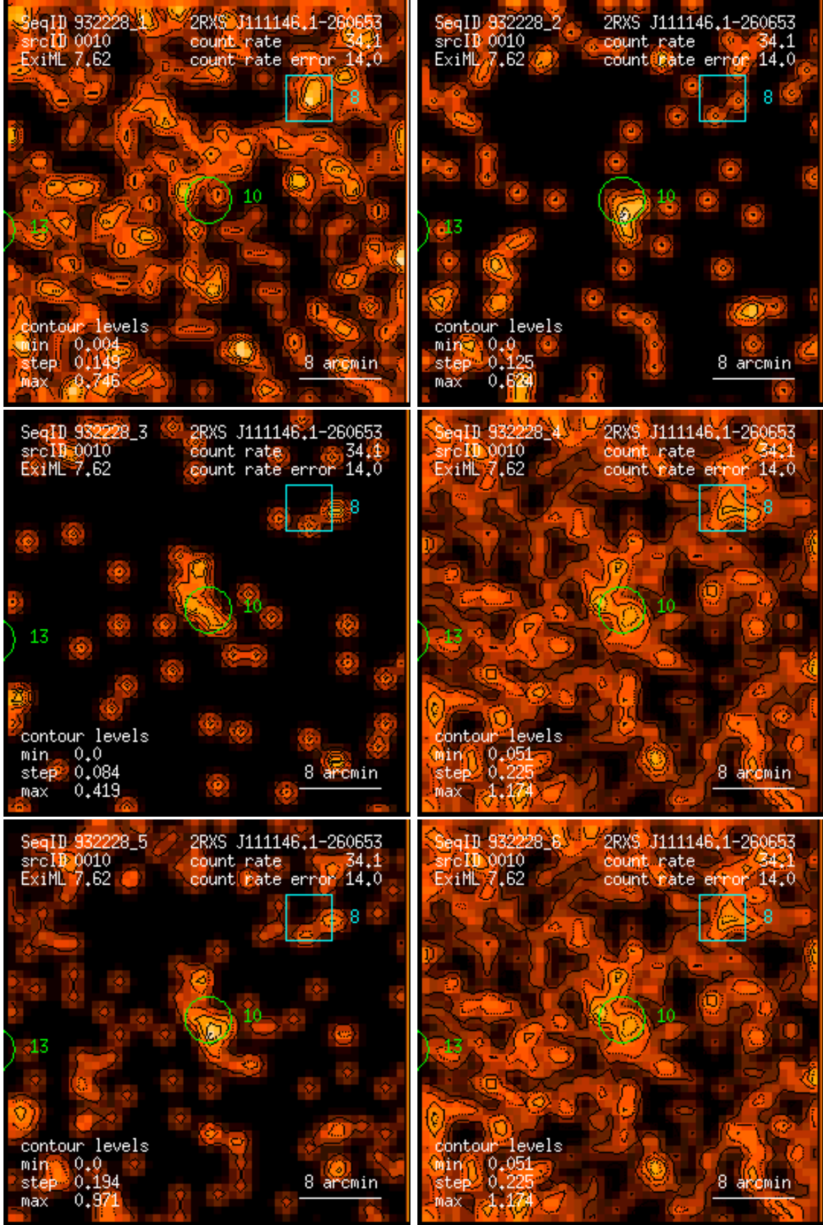
Figure 10: RASS 932228: detection 0010: band rate images, Gaussian filter: (1) PSPC channels 11 – 41, (2) 52 – 90, (3) 91 – 201, (4) 11 – 235, (5) 52 – 201, (6) 11 – 201. Broad band rates in counts/ks. Band rate contour levels in counts/ks/arcmin 2 .
