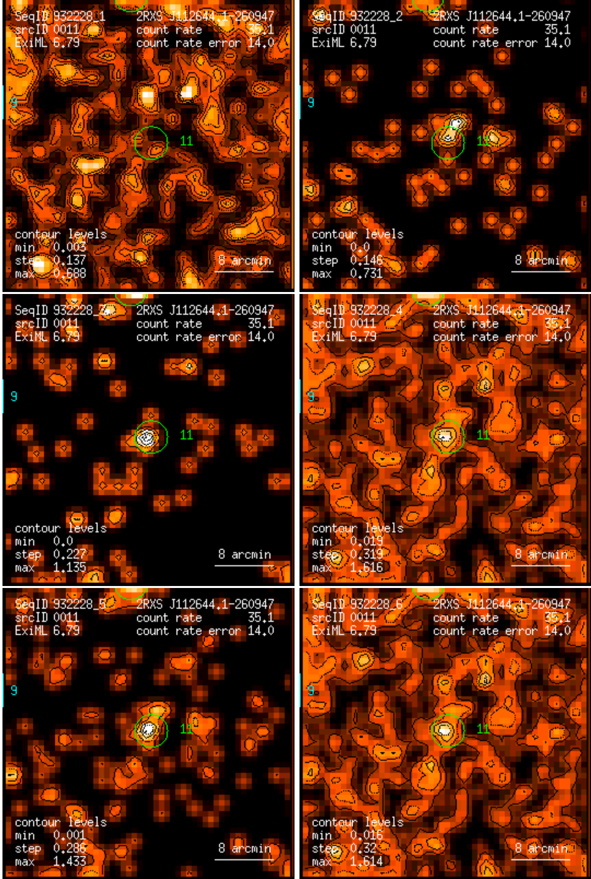
Figure 11: RASS 932228: detection 0011: band rate images, Gaussian filter: (1) PSPC channels 11 – 41, (2) 52 – 90, (3) 91 – 201, (4) 11 – 235, (5) 52 – 201, (6) 11 – 201. Broad band rates in counts/ks. Band rate contour levels in counts/ks/arcmin 2 .
