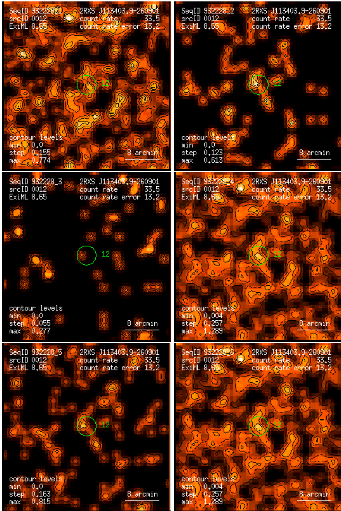
Figure 12: RASS 932228: detection 0012: band rate images, Gaussian filter: (1) PSPC channels 11 – 41, (2) 52 – 90, (3) 91 – 201, (4) 11 – 235, (5) 52 – 201, (6) 11 – 201. Broad band rates in counts/ks. Band rate contour levels in counts/ks/arcmin 2 .
