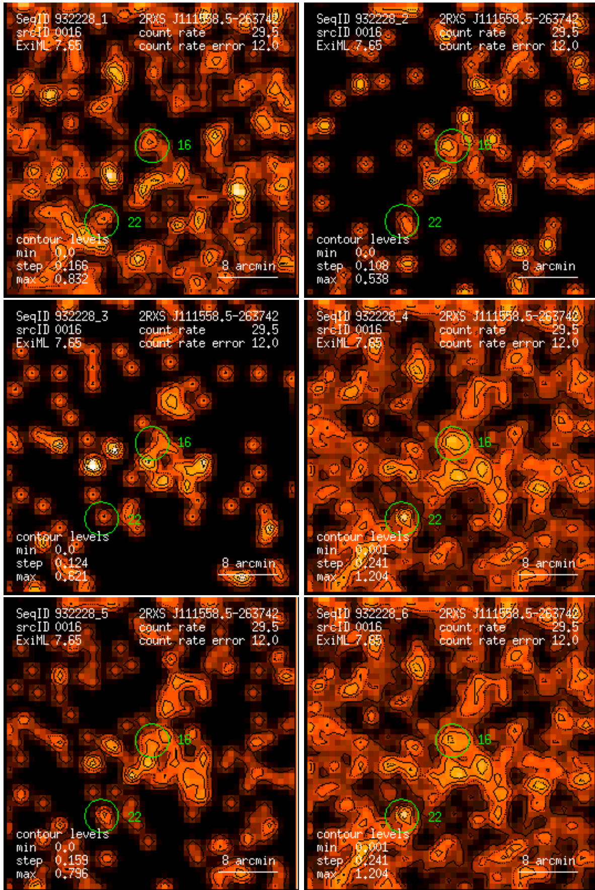
Figure 16: RASS 932228: detection 0016: band rate images, Gaussian filter: (1) PSPC channels 11 – 41, (2) 52 – 90, (3) 91 – 201, (4) 11 – 235, (5) 52 – 201, (6) 11 – 201. Broad band rates in counts/ks. Band rate contour levels in counts/ks/arcmin 2 .
