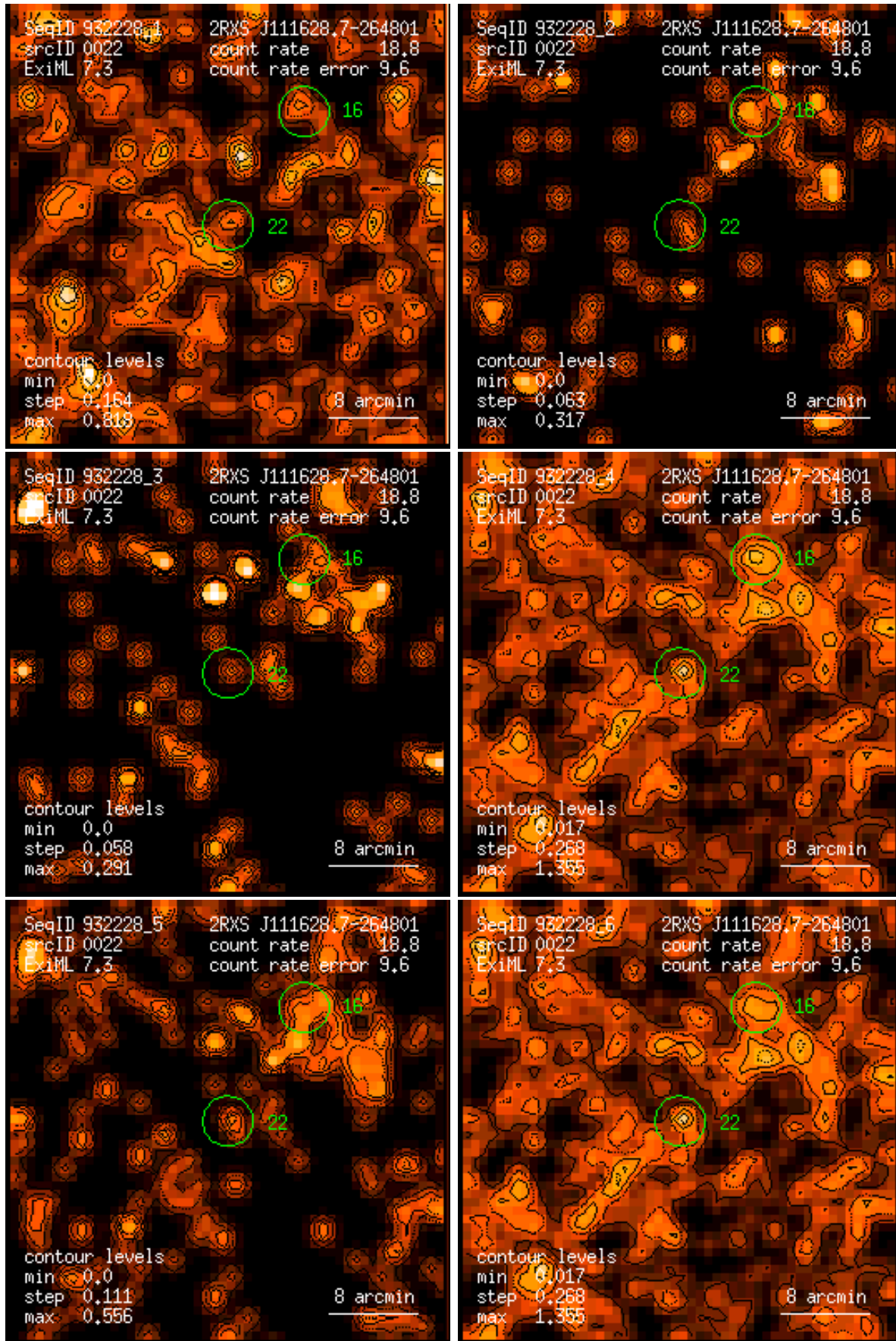
Figure 22: RASS 932228: detection 0022: band rate images, Gaussian filter: (1) PSPC channels 11 – 41, (2) 52 – 90, (3) 91 – 201, (4) 11 – 235, (5) 52 – 201, (6) 11 – 201. Broad band rates in counts/ks. Band rate contour levels in counts/ks/arcmin 2 .
