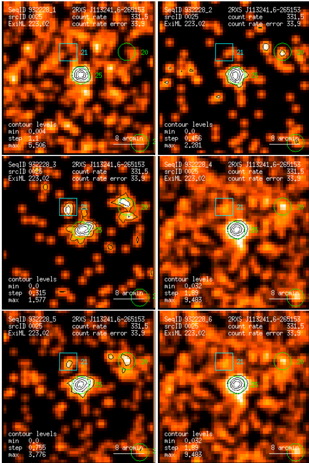
Figure 25: RASS 932228: detection 0025: band rate images, Gaussian filter: (1) PSPC channels 11 – 41, (2) 52 – 90, (3) 91 – 201, (4) 11 – 235, (5) 52 – 201, (6) 11 – 201. Broad band rates in counts/ks. Band rate contour levels in counts/ks/arcmin 2 .
