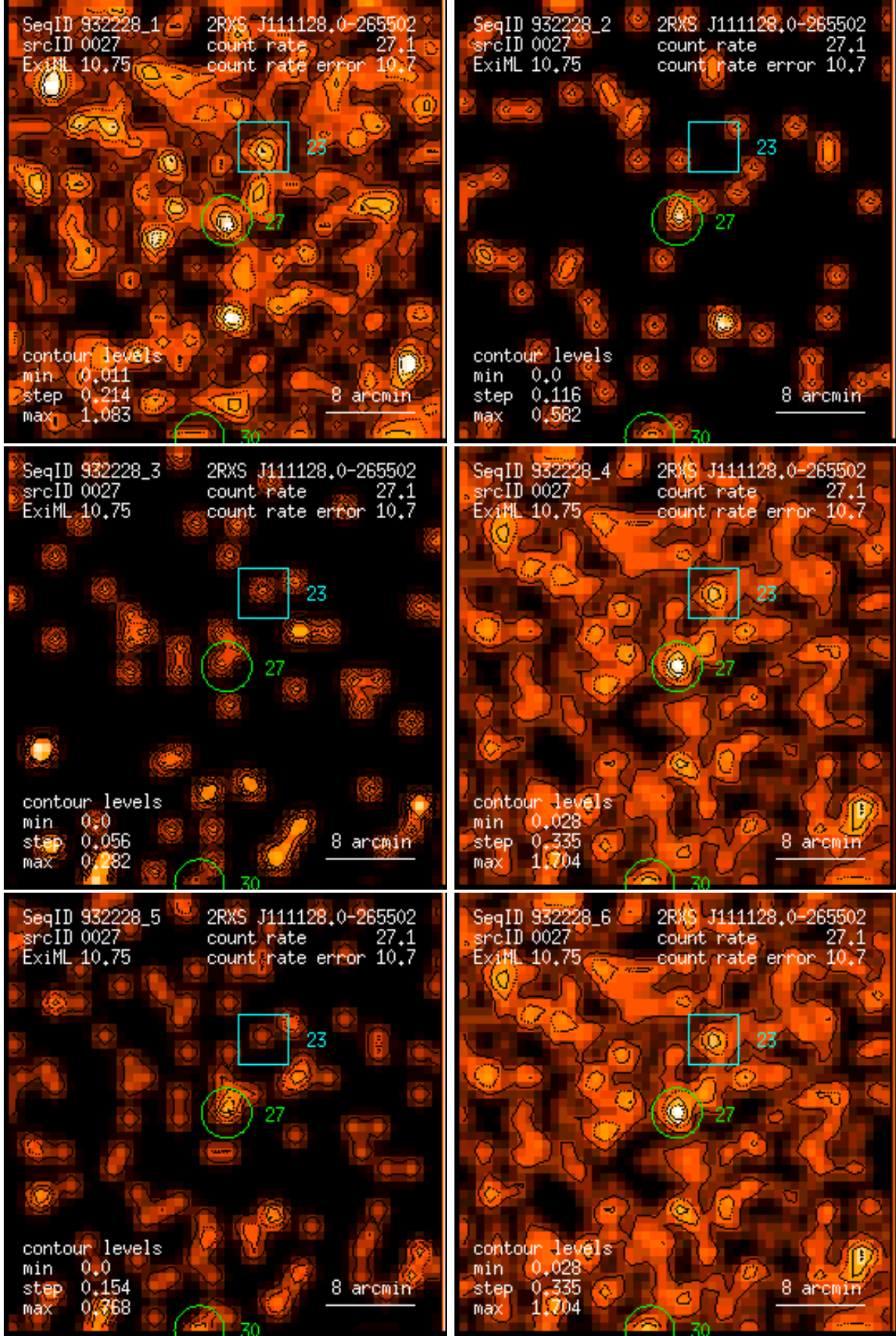
Figure 27: RASS 932228: detection 0027: band rate images, Gaussian filter: (1) PSPC channels 11 – 41, (2) 52 – 90, (3) 91 – 201, (4) 11 – 235, (5) 52 – 201, (6) 11 – 201. Broad band rates in counts/ks. Band rate contour levels in counts/ks/arcmin 2 .
