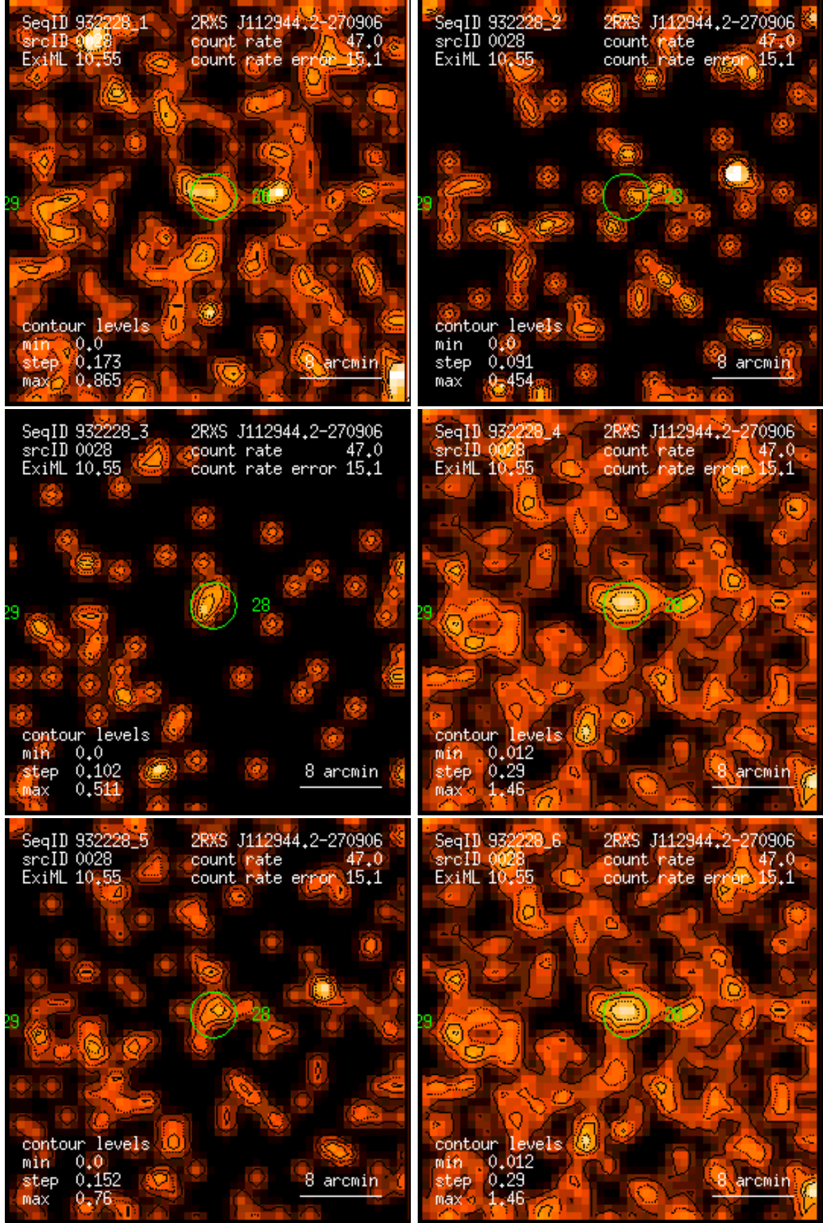
Figure 28: RASS 932228: detection 0028: band rate images, Gaussian filter: (1) PSPC channels 11 – 41, (2) 52 – 90, (3) 91 – 201, (4) 11 – 235, (5) 52 – 201, (6) 11 – 201. Broad band rates in counts/ks. Band rate contour levels in counts/ks/arcmin 2 .
