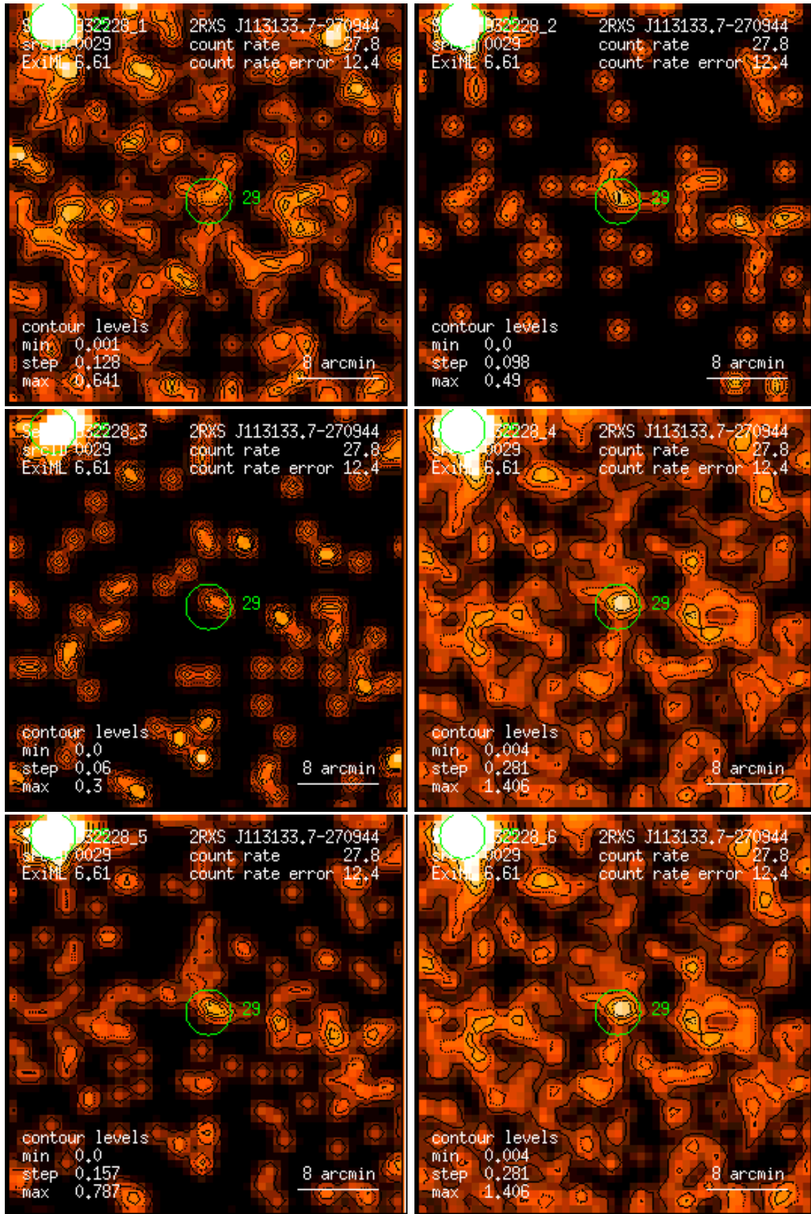
Figure 29: RASS 932228: detection 0029: band rate images, Gaussian filter: (1) PSPC channels 11 – 41, (2) 52 – 90, (3) 91 – 201, (4) 11 – 235, (5) 52 – 201, (6) 11 – 201. Broad band rates in counts/ks. Band rate contour levels in counts/ks/arcmin 2 .
