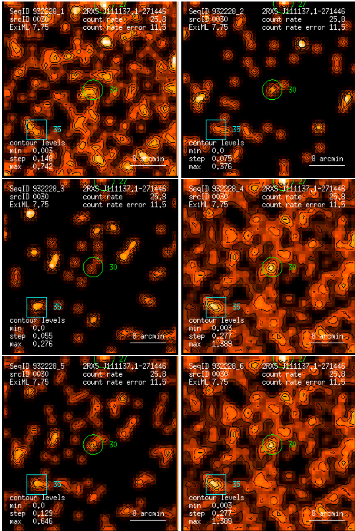
Figure 30: RASS 932228: detection 0030: band rate images, Gaussian filter: (1) PSPC channels 11 – 41, (2) 52 – 90, (3) 91 – 201, (4) 11 – 235, (5) 52 – 201, (6) 11 – 201. Broad band rates in counts/ks. Band rate contour levels in counts/ks/arcmin 2 .
