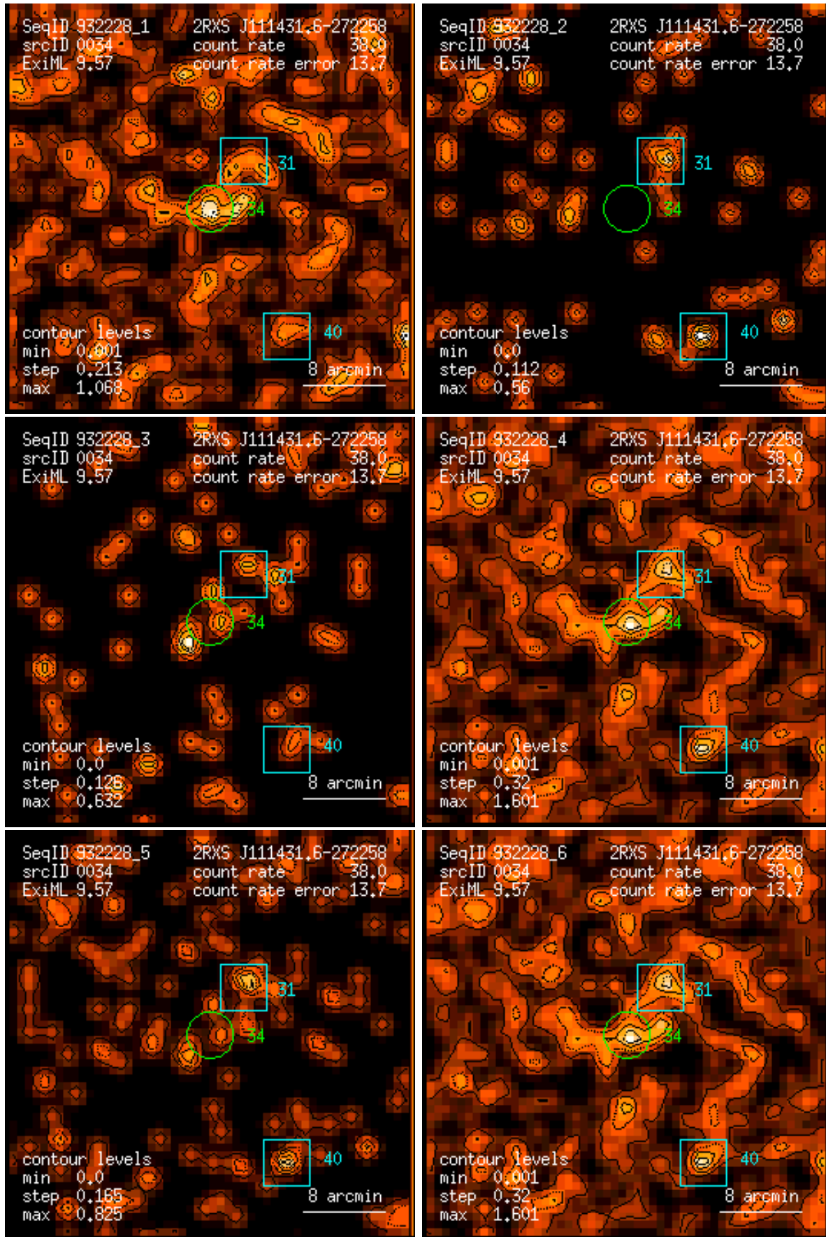
Figure 34: RASS 932228: detection 0034: band rate images, Gaussian filter: (1) PSPC channels 11 – 41, (2) 52 – 90, (3) 91 – 201, (4) 11 – 235, (5) 52 – 201, (6) 11 – 201. Broad band rates in counts/ks. Band rate contour levels in counts/ks/arcmin 2 .
