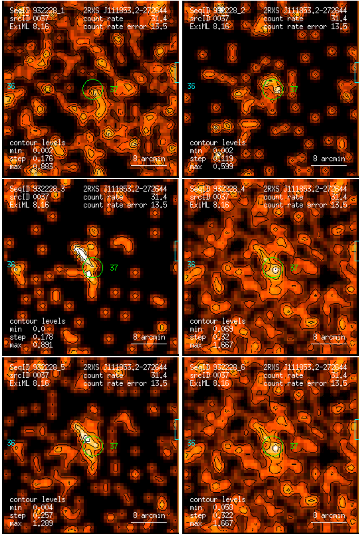
Figure 37: RASS 932228: detection 0037: band rate images, Gaussian filter: (1) PSPC channels 11 – 41, (2) 52 – 90, (3) 91 – 201, (4) 11 – 235, (5) 52 – 201, (6) 11 – 201. Broad band rates in counts/ks. Band rate contour levels in counts/ks/arcmin 2 .
