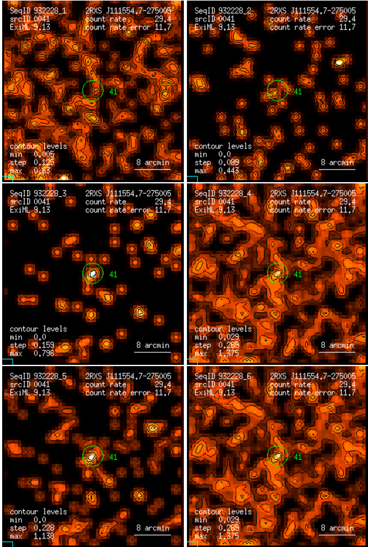
Figure 41: RASS 932228: detection 0041: band rate images, Gaussian filter: (1) PSPC channels 11 – 41, (2) 52 – 90, (3) 91 – 201, (4) 11 – 235, (5) 52 – 201, (6) 11 – 201. Broad band rates in counts/ks. Band rate contour levels in counts/ks/arcmin 2 .
