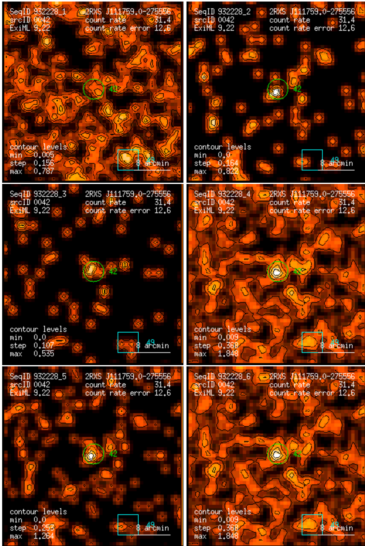
Figure 42: RASS 932228: detection 0042: band rate images, Gaussian filter: (1) PSPC channels 11 – 41, (2) 52 – 90, (3) 91 – 201, (4) 11 – 235, (5) 52 – 201, (6) 11 – 201. Broad band rates in counts/ks. Band rate contour levels in counts/ks/arcmin 2 .
