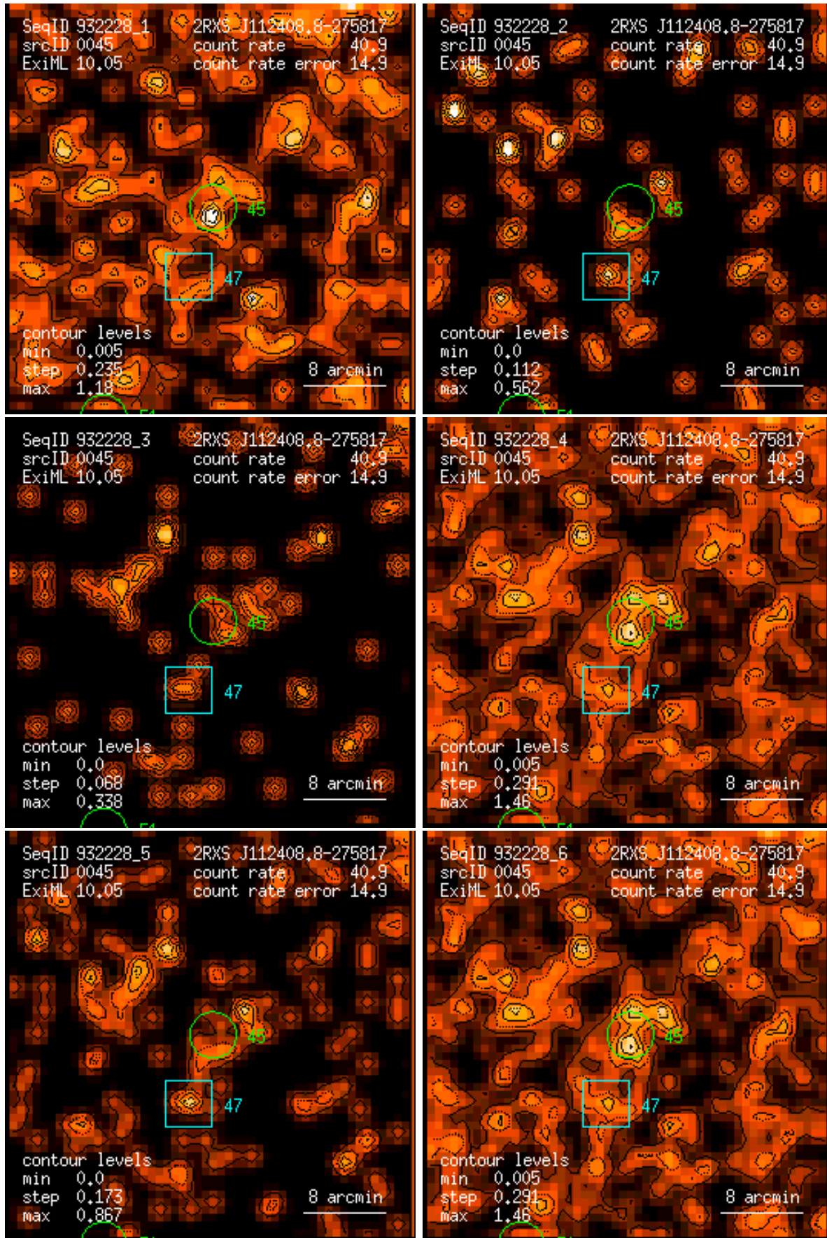
Figure 45: RASS 932228: detection 0045: band rate images, Gaussian filter: (1) PSPC channels 11 – 41, (2) 52 – 90, (3) 91 – 201, (4) 11 – 235, (5) 52 – 201, (6) 11 – 201. Broad band rates in counts/ks. Band rate contour levels in counts/ks/arcmin 2 .
