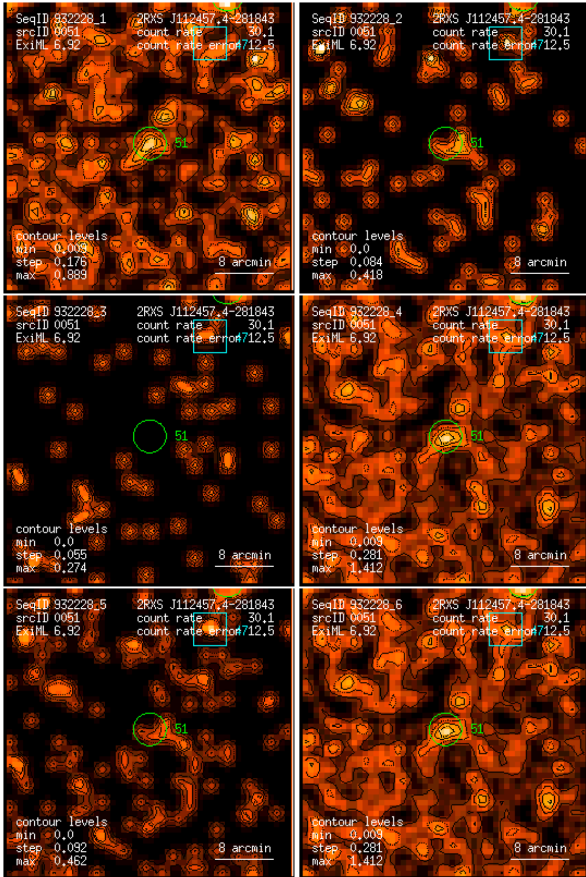
Figure 51: RASS 932228: detection 0051: band rate images, Gaussian filter: (1) PSPC channels 11 – 41, (2) 52 – 90, (3) 91 – 201, (4) 11 – 235, (5) 52 – 201, (6) 11 – 201. Broad band rates in counts/ks. Band rate contour levels in counts/ks/arcmin 2 .
