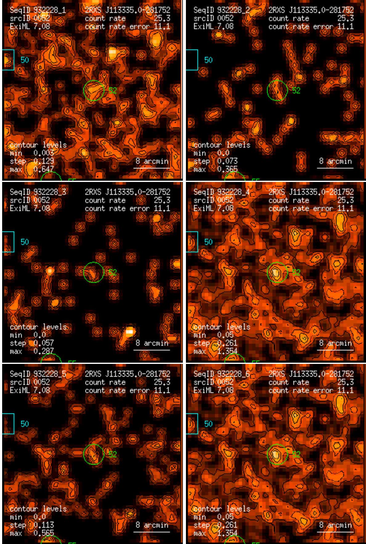
Figure 52: RASS 932228: detection 0052: band rate images, Gaussian filter: (1) PSPC channels 11 – 41, (2) 52 – 90, (3) 91 – 201, (4) 11 – 235, (5) 52 – 201, (6) 11 – 201. Broad band rates in counts/ks. Band rate contour levels in counts/ks/arcmin 2 .
