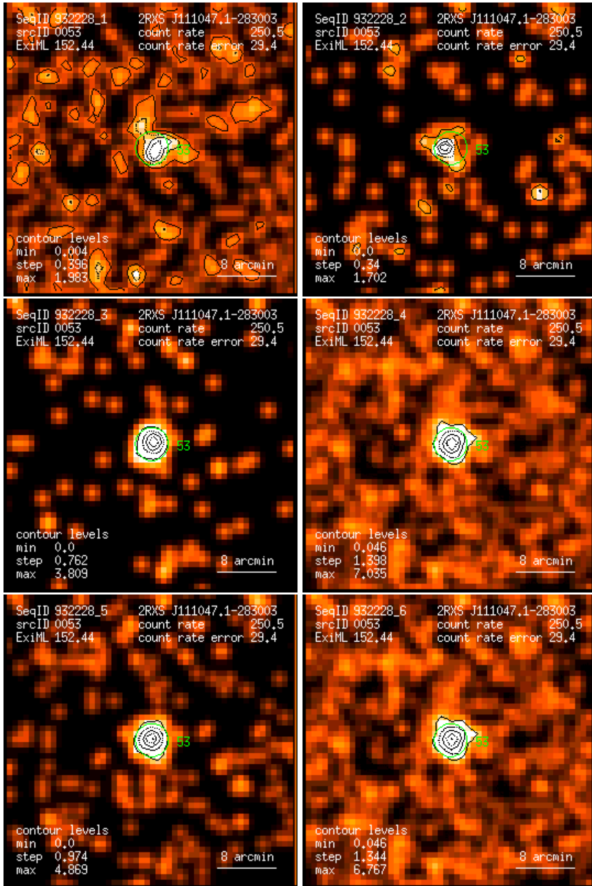
Figure 53: RASS 932228: detection 0053: band rate images, Gaussian filter: (1) PSPC channels 11 – 41, (2) 52 – 90, (3) 91 – 201, (4) 11 – 235, (5) 52 – 201, (6) 11 – 201. Broad band rates in counts/ks. Band rate contour levels in counts/ks/arcmin 2 .
