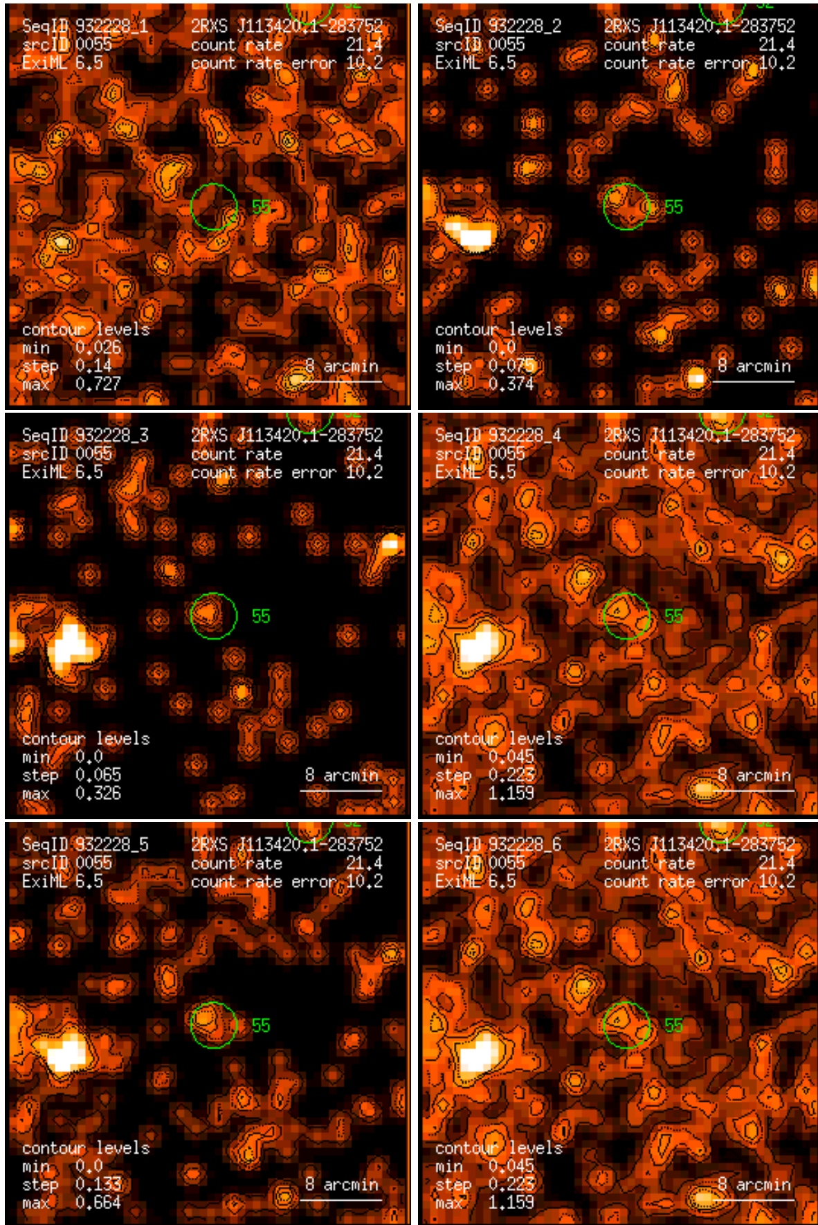
Figure 55: RASS 932228: detection 0055: band rate images, Gaussian filter: (1) PSPC channels 11 – 41, (2) 52 – 90, (3) 91 – 201, (4) 11 – 235, (5) 52 – 201, (6) 11 – 201. Broad band rates in counts/ks. Band rate contour levels in counts/ks/arcmin 2 .
