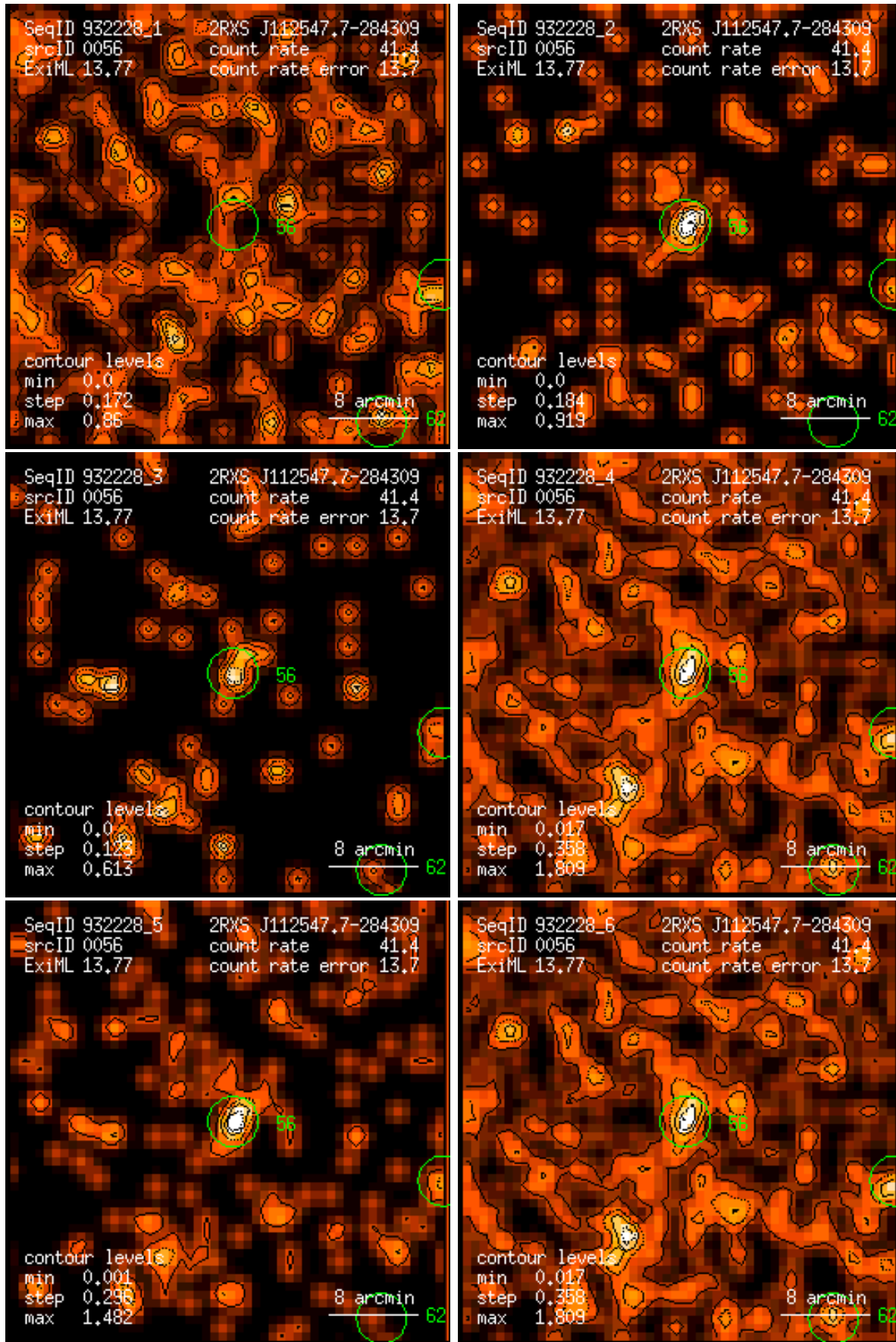
Figure 56: RASS 932228: detection 0056: band rate images, Gaussian filter: (1) PSPC channels 11 – 41, (2) 52 – 90, (3) 91 – 201, (4) 11 – 235, (5) 52 – 201, (6) 11 – 201. Broad band rates in counts/ks. Band rate contour levels in counts/ks/arcmin 2 .
