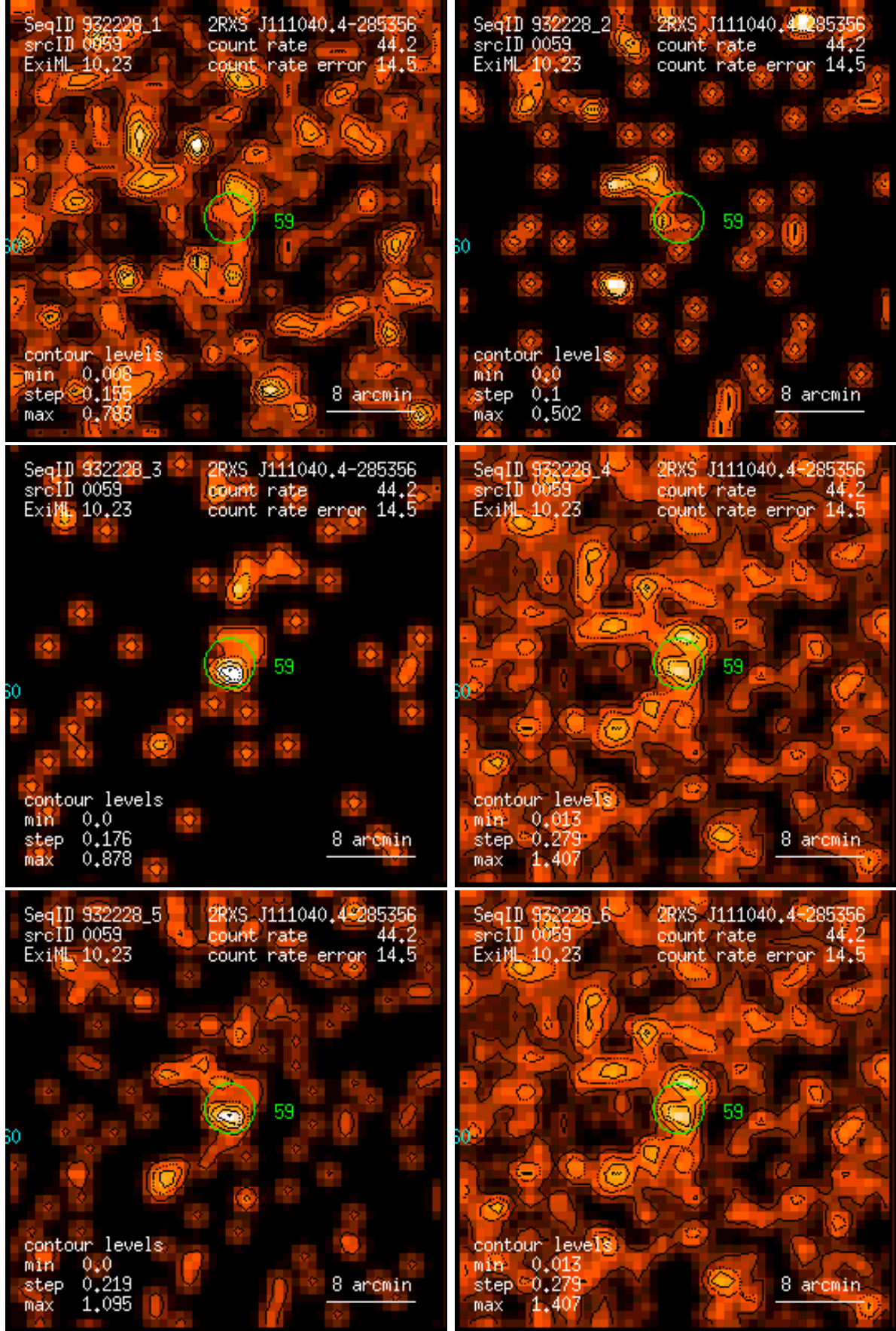
Figure 59: RASS 932228: detection 0059: band rate images, Gaussian filter: (1) PSPC channels 11 – 41, (2) 52 – 90, (3) 91 – 201, (4) 11 – 235, (5) 52 – 201, (6) 11 – 201. Broad band rates in counts/ks. Band rate contour levels in counts/ks/arcmin 2 .
