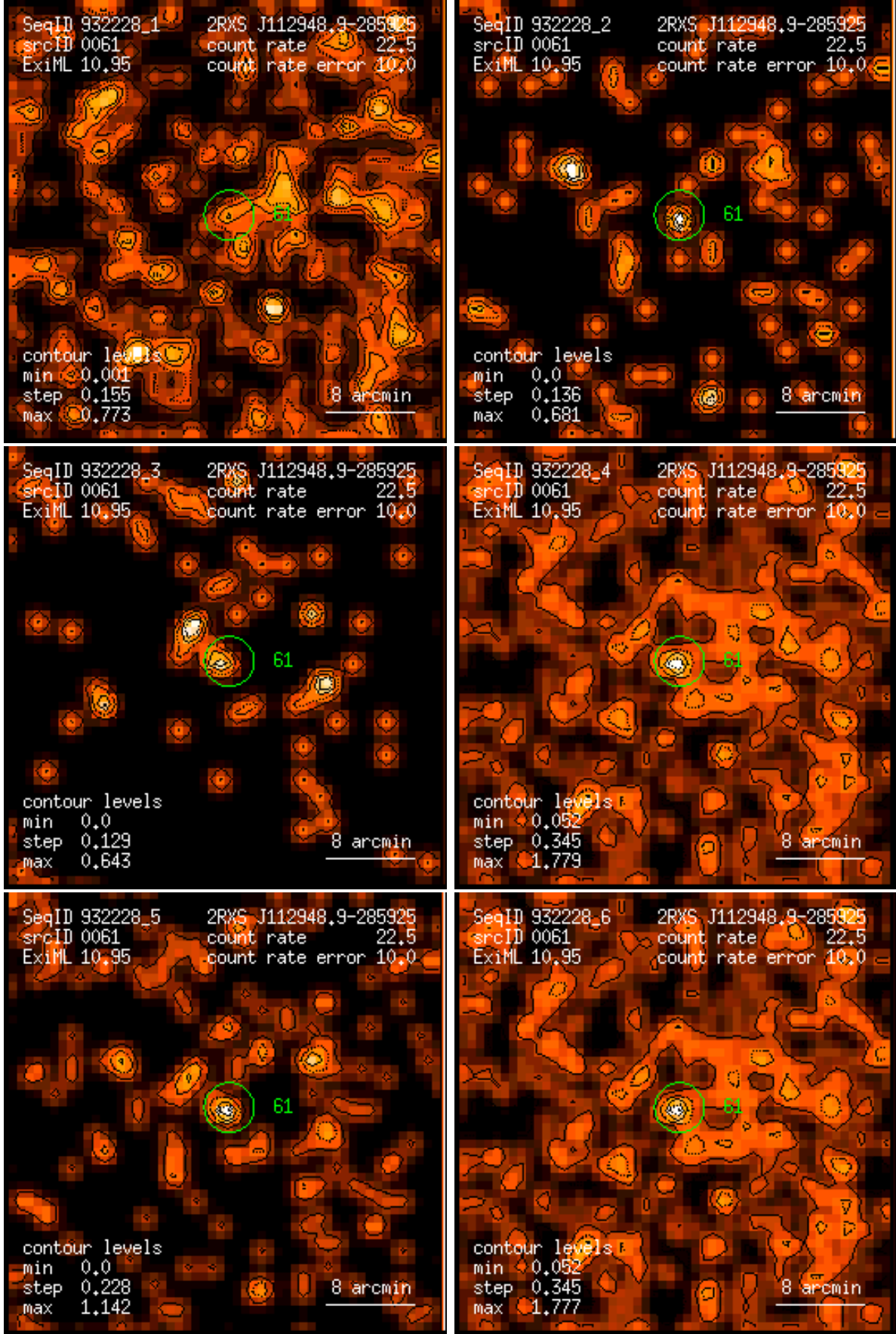
Figure 61: RASS 932228: detection 0061: band rate images, Gaussian filter: (1) PSPC channels 11 – 41, (2) 52 – 90, (3) 91 – 201, (4) 11 – 235, (5) 52 – 201, (6) 11 – 201. Broad band rates in counts/ks. Band rate contour levels in counts/ks/arcmin 2 .
