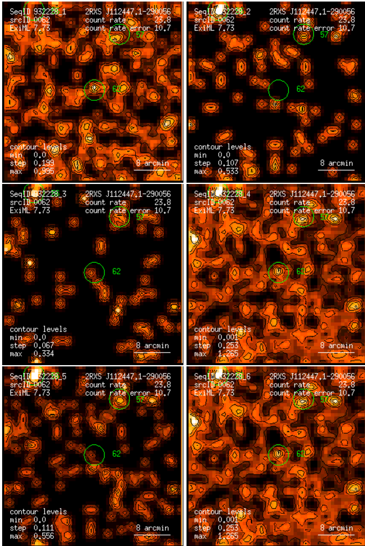
Figure 62: RASS 932228: detection 0062: band rate images, Gaussian filter: (1) PSPC channels 11 – 41, (2) 52 – 90, (3) 91 – 201, (4) 11 – 235, (5) 52 – 201, (6) 11 – 201. Broad band rates in counts/ks. Band rate contour levels in counts/ks/arcmin 2 .
