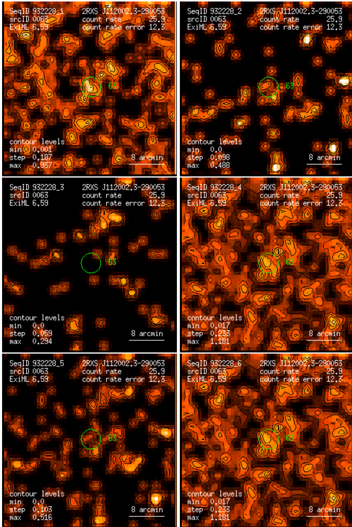
Figure 63: RASS 932228: detection 0063: band rate images, Gaussian filter: (1) PSPC channels 11 – 41, (2) 52 – 90, (3) 91 – 201, (4) 11 – 235, (5) 52 – 201, (6) 11 – 201. Broad band rates in counts/ks. Band rate contour levels in counts/ks/arcmin 2 .
