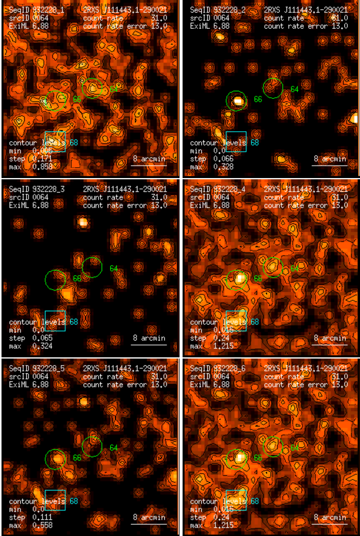
Figure 64: RASS 932228: detection 0064: band rate images, Gaussian filter: (1) PSPC channels 11 – 41, (2) 52 – 90, (3) 91 – 201, (4) 11 – 235, (5) 52 – 201, (6) 11 – 201. Broad band rates in counts/ks. Band rate contour levels in counts/ks/arcmin 2 .
