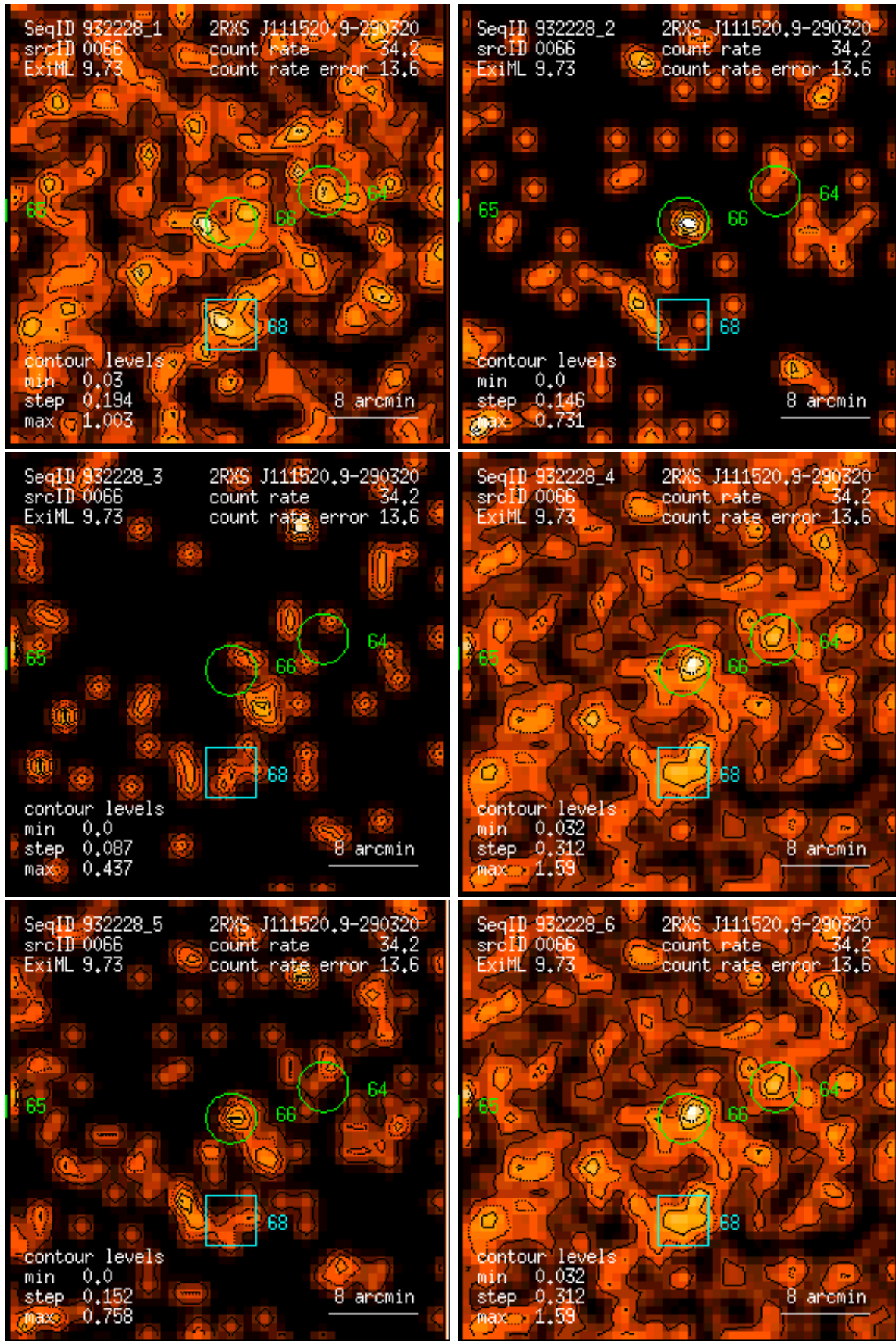
Figure 66: RASS 932228: detection 0066: band rate images, Gaussian filter: (1) PSPC channels 11 – 41, (2) 52 – 90, (3) 91 – 201, (4) 11 – 235, (5) 52 – 201, (6) 11 – 201. Broad band rates in counts/ks. Band rate contour levels in counts/ks/arcmin 2 .
