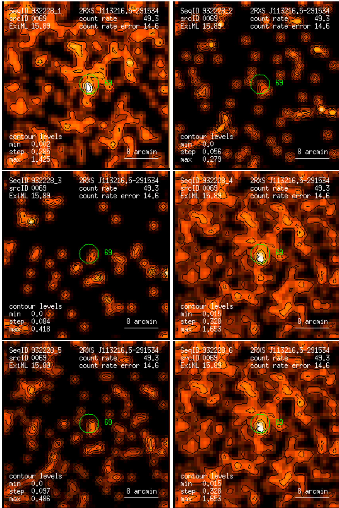
Figure 69: RASS 932228: detection 0069: band rate images, Gaussian filter: (1) PSPC channels 11 – 41, (2) 52 – 90, (3) 91 – 201, (4) 11 – 235, (5) 52 – 201, (6) 11 – 201. Broad band rates in counts/ks. Band rate contour levels in counts/ks/arcmin 2 .
