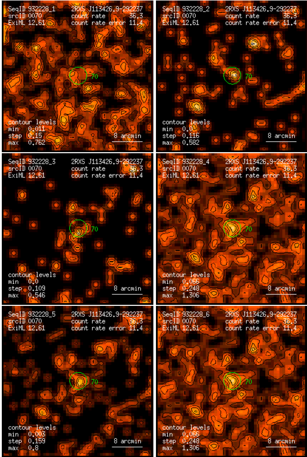
Figure 70: RASS 932228: detection 0070: band rate images, Gaussian filter: (1) PSPC channels 11 – 41, (2) 52 – 90, (3) 91 – 201, (4) 11 – 235, (5) 52 – 201, (6) 11 – 201. Broad band rates in counts/ks. Band rate contour levels in counts/ks/arcmin 2 .
