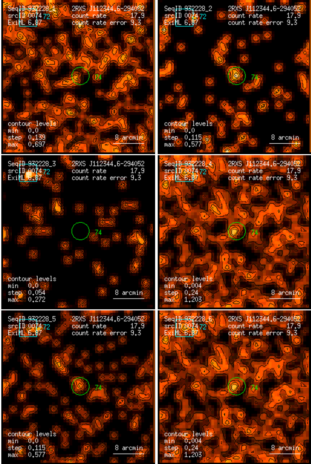
Figure 74: RASS 932228: detection 0074: band rate images, Gaussian filter: (1) PSPC channels 11 – 41, (2) 52 – 90, (3) 91 – 201, (4) 11 – 235, (5) 52 – 201, (6) 11 – 201. Broad band rates in counts/ks. Band rate contour levels in counts/ks/arcmin 2 .
