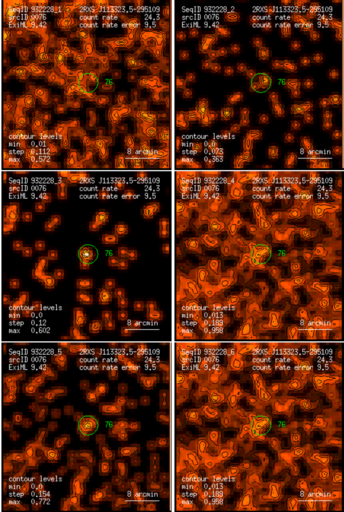
Figure 76: RASS 932228: detection 0076: band rate images, Gaussian filter: (1) PSPC channels 11 – 41, (2) 52 – 90, (3) 91 – 201, (4) 11 – 235, (5) 52 – 201, (6) 11 – 201. Broad band rates in counts/ks. Band rate contour levels in counts/ks/arcmin 2 .
