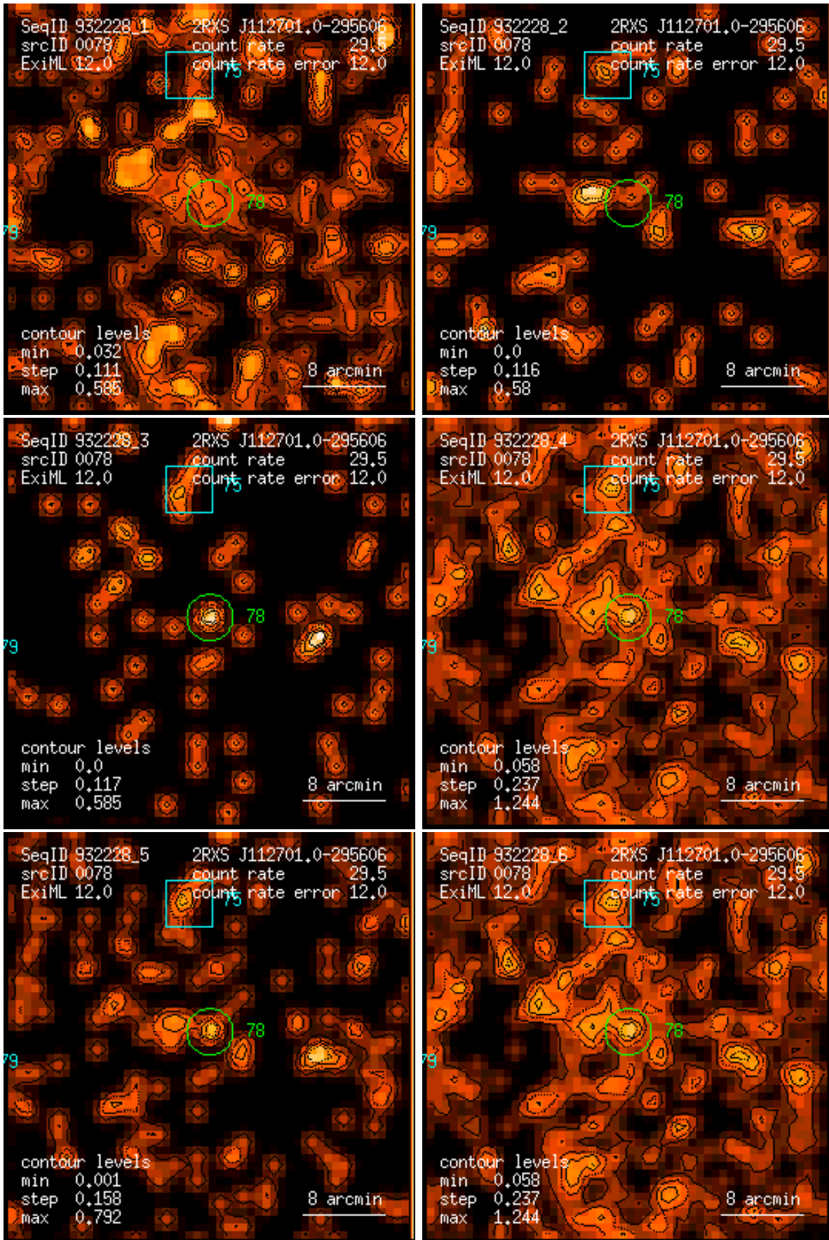
Figure 78: RASS 932228: detection 0078: band rate images, Gaussian filter: (1) PSPC channels 11 – 41, (2) 52 – 90, (3) 91 – 201, (4) 11 – 235, (5) 52 – 201, (6) 11 – 201. Broad band rates in counts/ks. Band rate contour levels in counts/ks/arcmin 2 .
