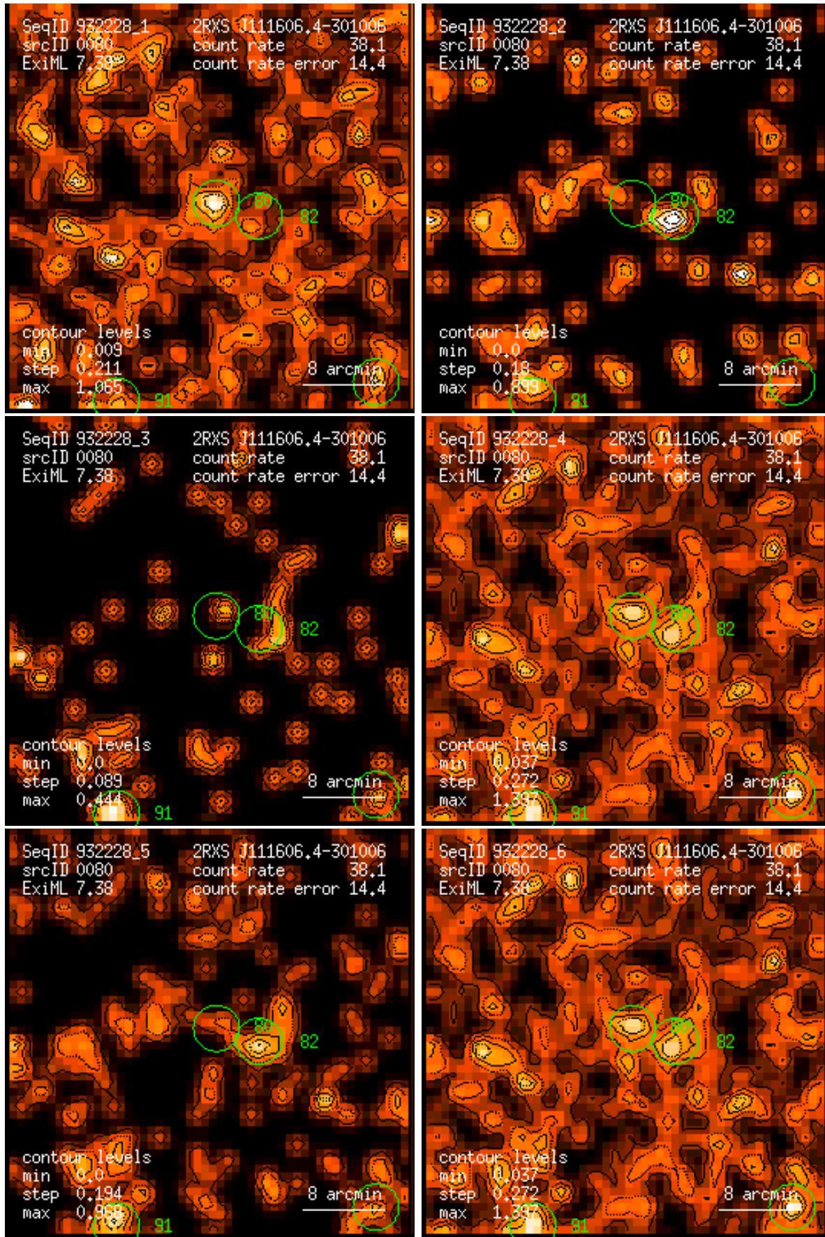
Figure 80: RASS 932228: detection 0080: band rate images, Gaussian filter: (1) PSPC channels 11 – 41, (2) 52 – 90, (3) 91 – 201, (4) 11 – 235, (5) 52 – 201, (6) 11 – 201. Broad band rates in counts/ks. Band rate contour levels in counts/ks/arcmin 2 .
