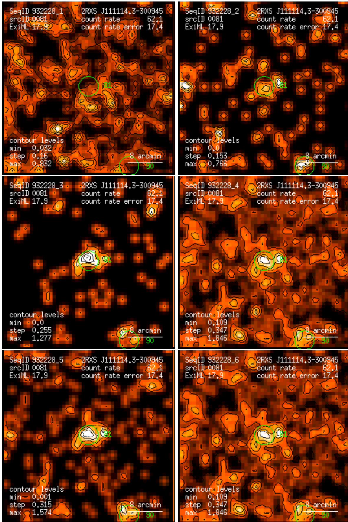
Figure 81: RASS 932228: detection 0081: band rate images, Gaussian filter: (1) PSPC channels 11 – 41, (2) 52 – 90, (3) 91 – 201, (4) 11 – 235, (5) 52 – 201, (6) 11 – 201. Broad band rates in counts/ks. Band rate contour levels in counts/ks/arcmin 2 .
