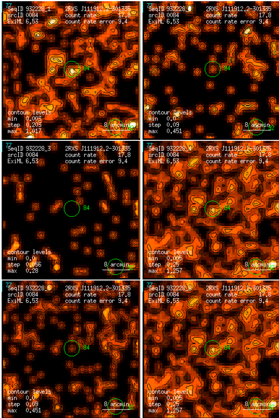
Figure 84: RASS 932228: detection 0084: band rate images, Gaussian filter: (1) PSPC channels 11 – 41, (2) 52 – 90, (3) 91 – 201, (4) 11 – 235, (5) 52 – 201, (6) 11 – 201. Broad band rates in counts/ks. Band rate contour levels in counts/ks/arcmin 2 .
