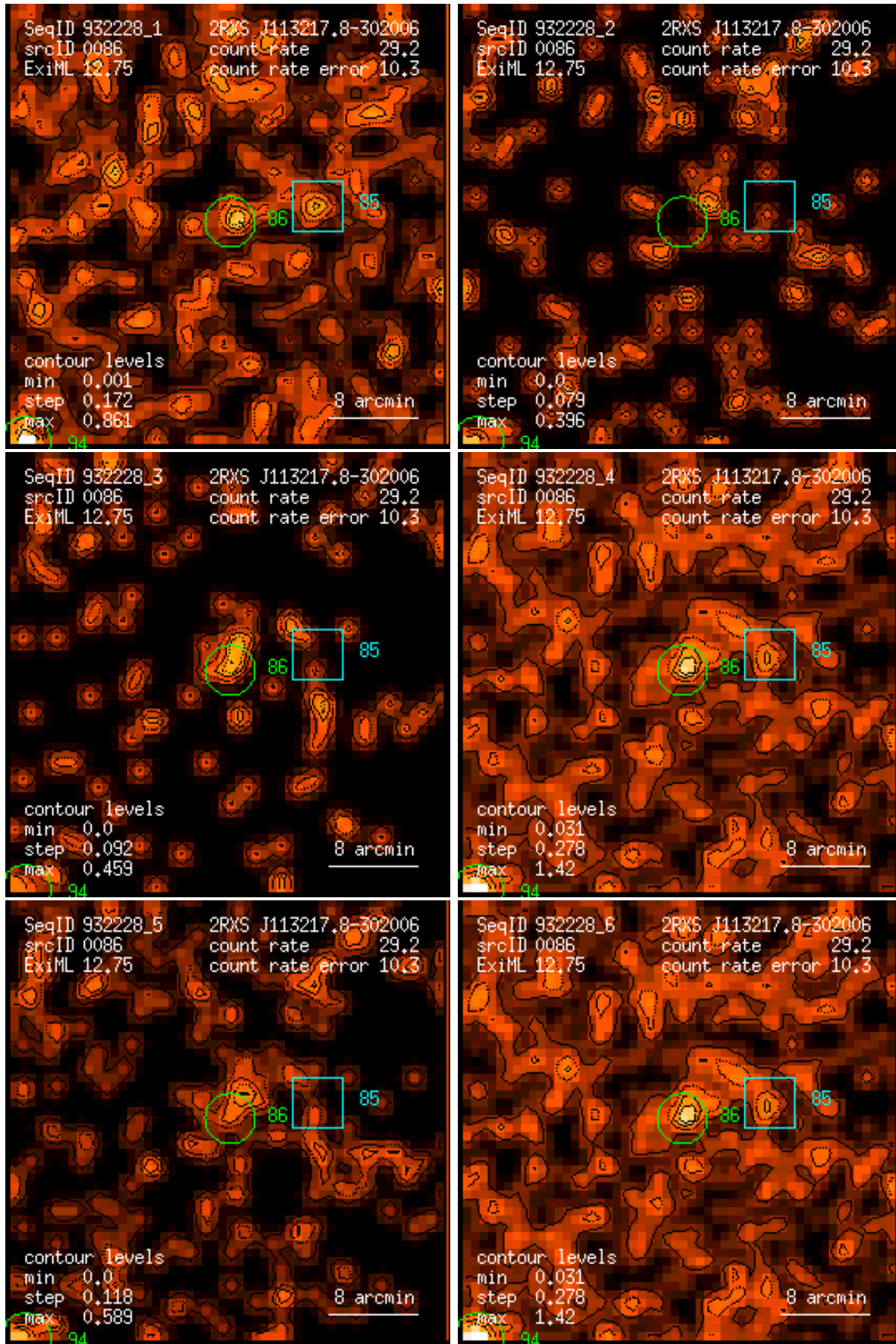
Figure 86: RASS 932228: detection 0086: band rate images, Gaussian filter: (1) PSPC channels 11 – 41, (2) 52 – 90, (3) 91 – 201, (4) 11 – 235, (5) 52 – 201, (6) 11 – 201. Broad band rates in counts/ks. Band rate contour levels in counts/ks/arcmin 2 .
