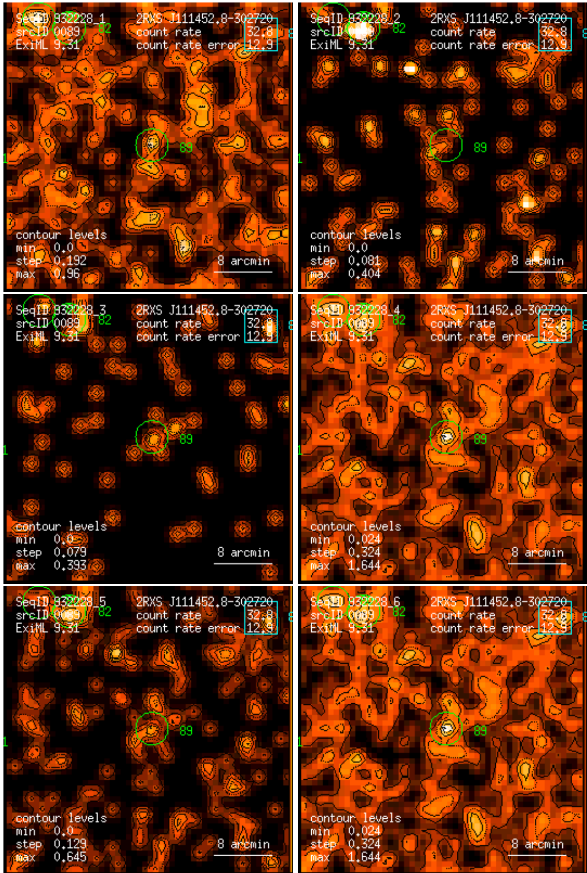
Figure 89: RASS 932228: detection 0089: band rate images, Gaussian filter: (1) PSPC channels 11 – 41, (2) 52 – 90, (3) 91 – 201, (4) 11 – 235, (5) 52 – 201, (6) 11 – 201. Broad band rates in counts/ks. Band rate contour levels in counts/ks/arcmin 2 .
