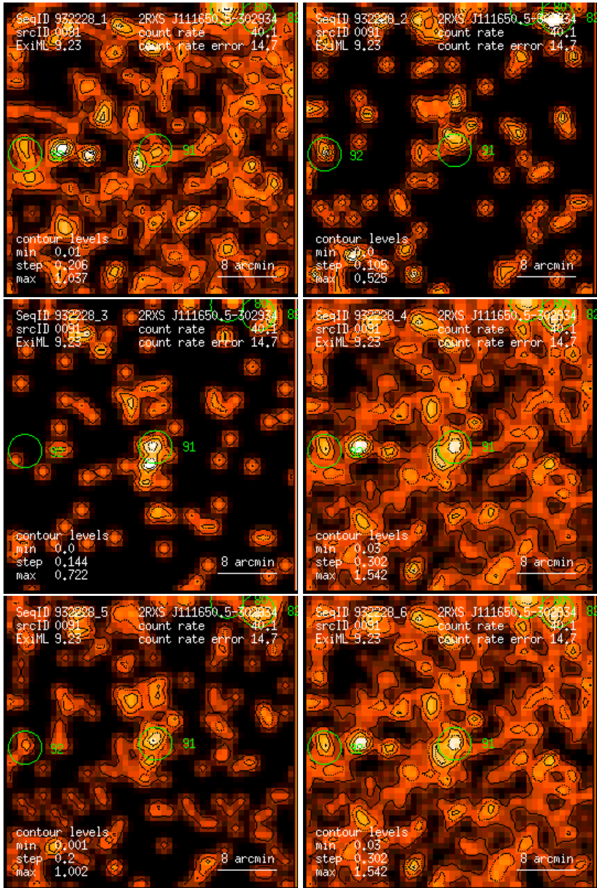
Figure 91: RASS 932228: detection 0091: band rate images, Gaussian filter: (1) PSPC channels 11 – 41, (2) 52 – 90, (3) 91 – 201, (4) 11 – 235, (5) 52 – 201, (6) 11 – 201. Broad band rates in counts/ks. Band rate contour levels in counts/ks/arcmin 2 .
