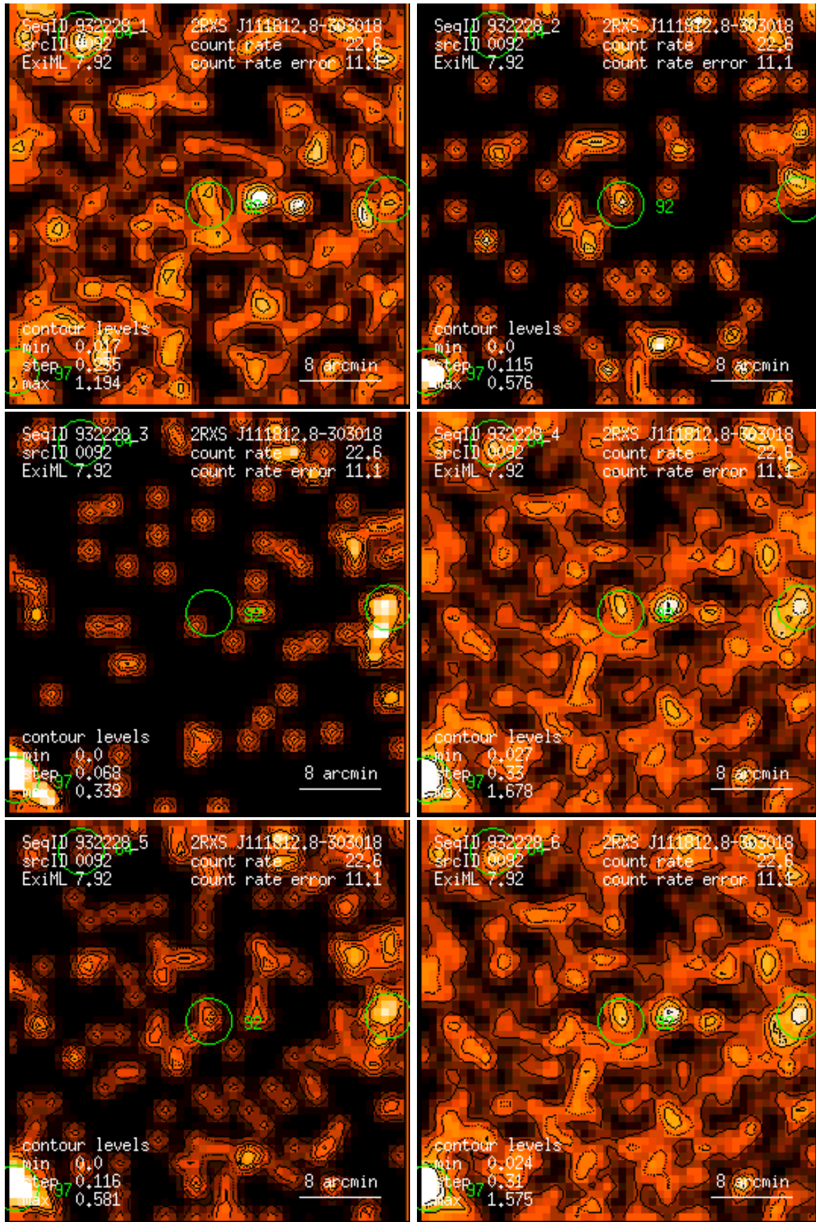
Figure 92: RASS 932228: detection 0092: band rate images, Gaussian filter: (1) PSPC channels 11 – 41, (2) 52 – 90, (3) 91 – 201, (4) 11 – 235, (5) 52 – 201, (6) 11 – 201. Broad band rates in counts/ks. Band rate contour levels in counts/ks/arcmin 2 .
