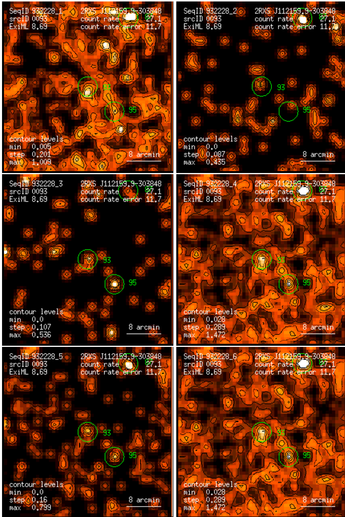
Figure 93: RASS 932228: detection 0093: band rate images, Gaussian filter: (1) PSPC channels 11 – 41, (2) 52 – 90, (3) 91 – 201, (4) 11 – 235, (5) 52 – 201, (6) 11 – 201. Broad band rates in counts/ks. Band rate contour levels in counts/ks/arcmin 2 .
