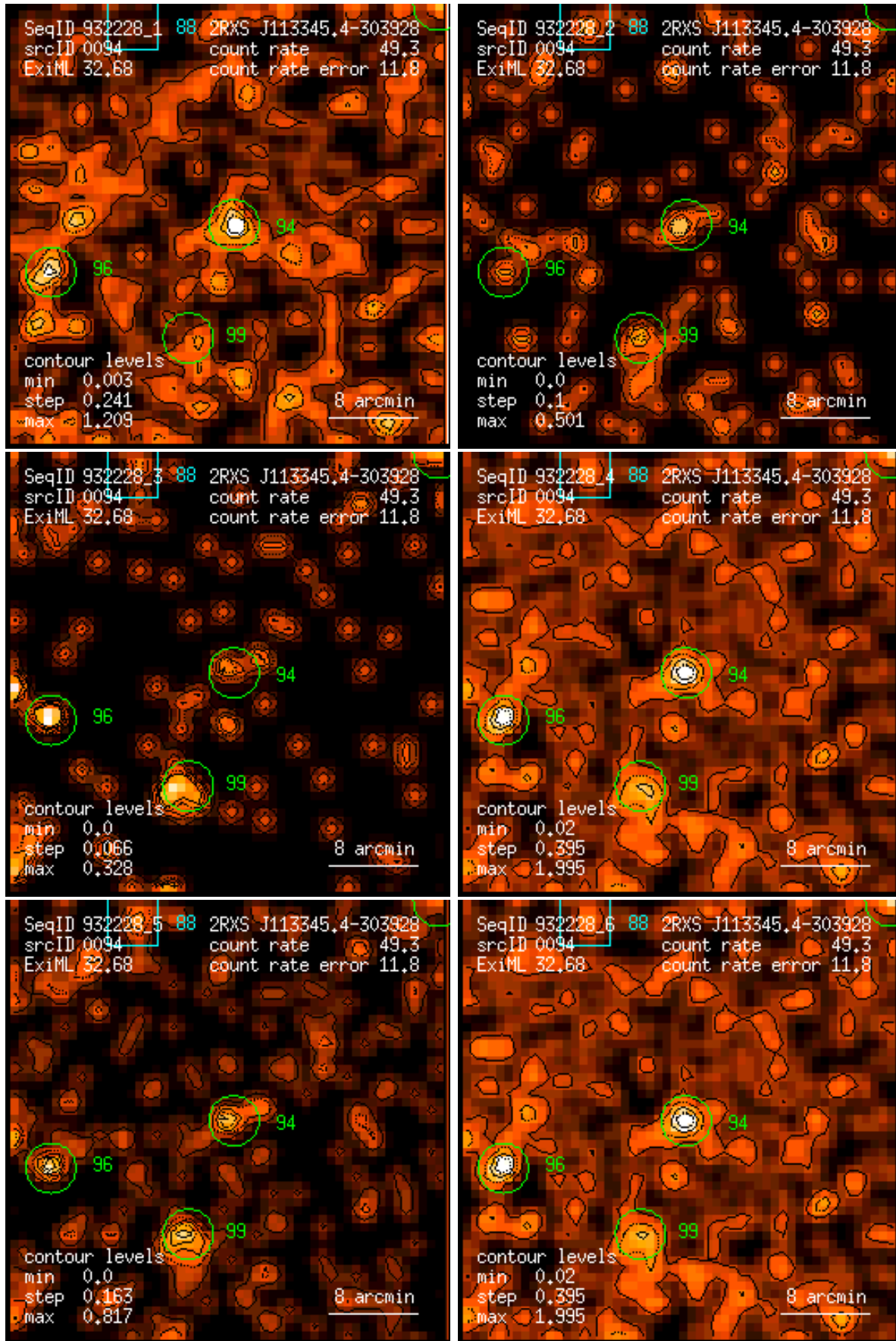
Figure 94: RASS 932228: detection 0094: band rate images, Gaussian filter: (1) PSPC channels 11 – 41, (2) 52 – 90, (3) 91 – 201, (4) 11 – 235, (5) 52 – 201, (6) 11 – 201. Broad band rates in counts/ks. Band rate contour levels in counts/ks/arcmin 2 .
