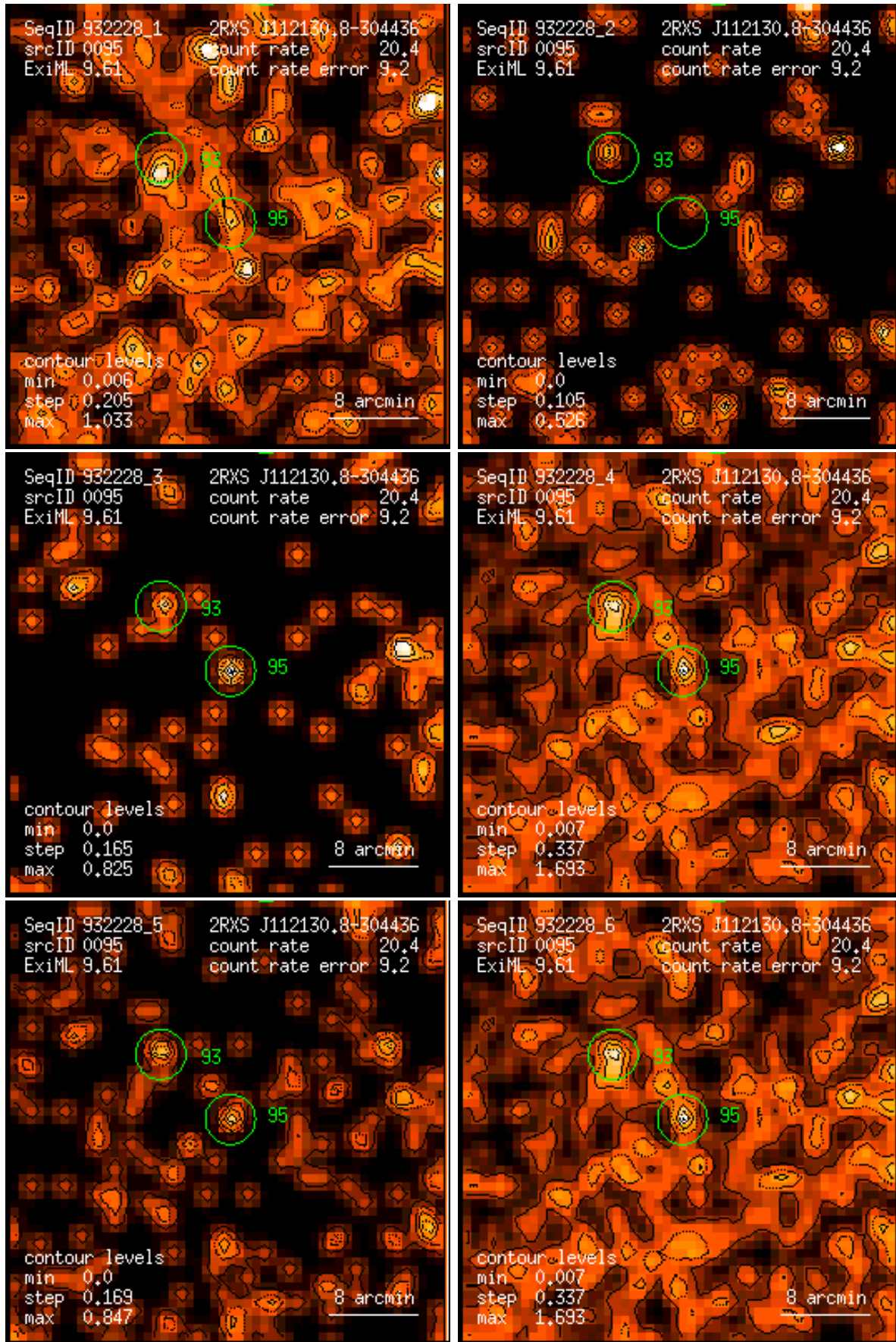
Figure 95: RASS 932228: detection 0095: band rate images, Gaussian filter: (1) PSPC channels 11 – 41, (2) 52 – 90, (3) 91 – 201, (4) 11 – 235, (5) 52 – 201, (6) 11 – 201. Broad band rates in counts/ks. Band rate contour levels in counts/ks/arcmin 2 .
