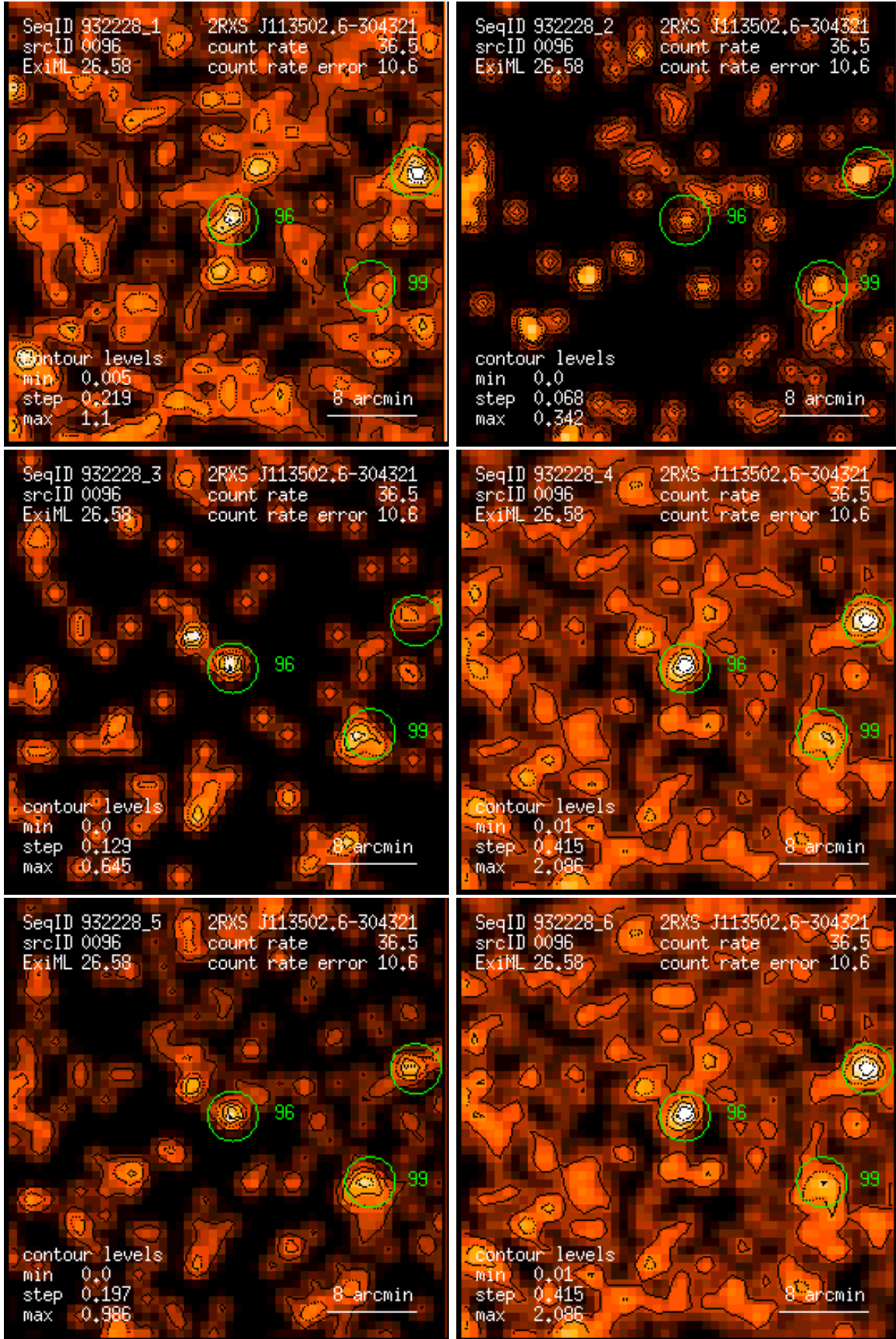
Figure 96: RASS 932228: detection 0096: band rate images, Gaussian filter: (1) PSPC channels 11 – 41, (2) 52 – 90, (3) 91 – 201, (4) 11 – 235, (5) 52 – 201, (6) 11 – 201. Broad band rates in counts/ks. Band rate contour levels in counts/ks/arcmin 2 .
