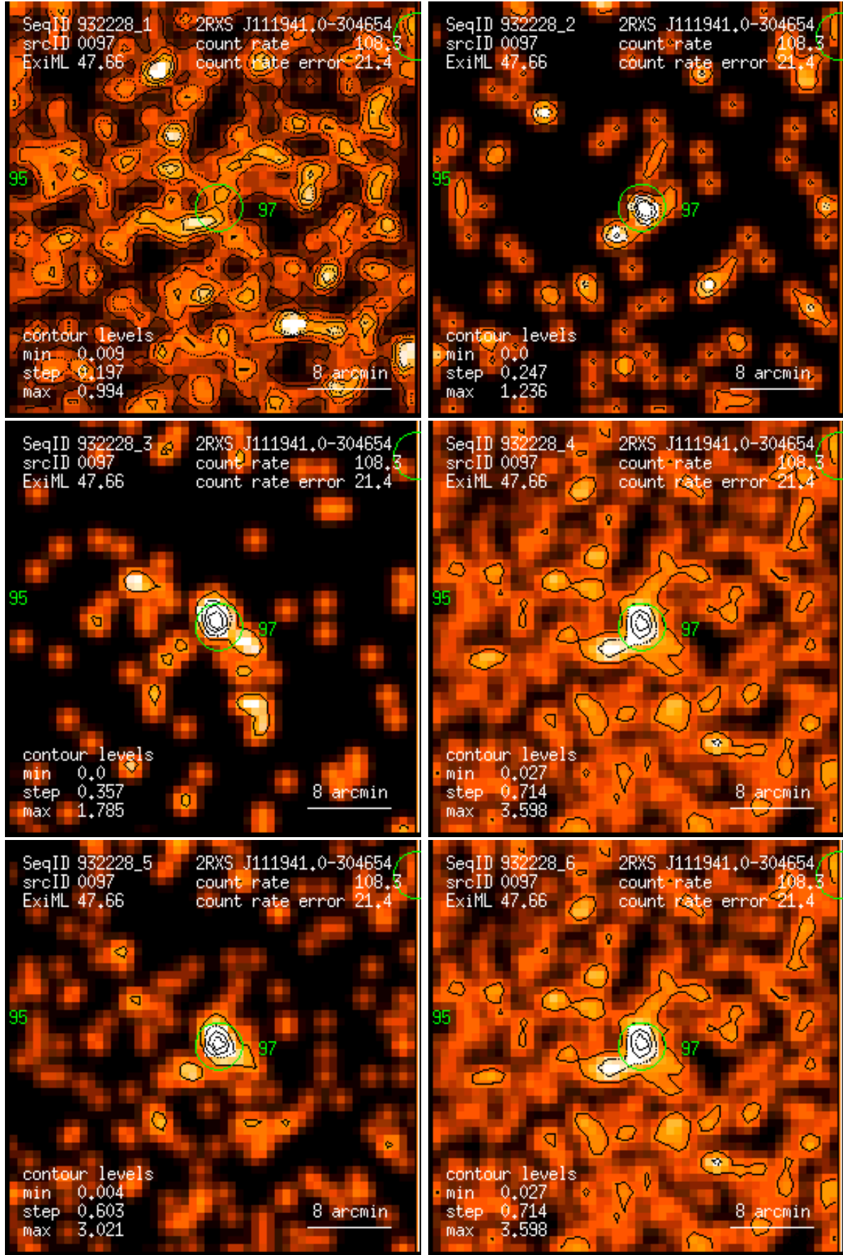
Figure 97: RASS 932228: detection 0097: band rate images, Gaussian filter: (1) PSPC channels 11 – 41, (2) 52 – 90, (3) 91 – 201, (4) 11 – 235, (5) 52 – 201, (6) 11 – 201. Broad band rates in counts/ks. Band rate contour levels in counts/ks/arcmin 2 .
