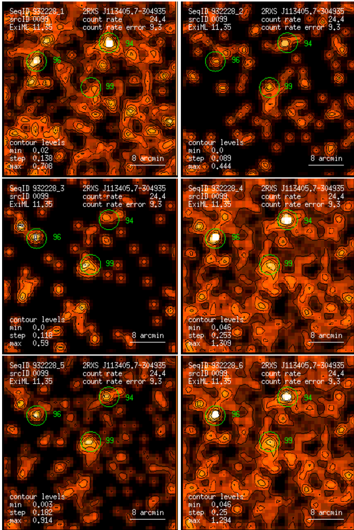
Figure 99: RASS 932228: detection 0099: band rate images, Gaussian filter: (1) PSPC channels 11 – 41, (2) 52 – 90, (3) 91 – 201, (4) 11 – 235, (5) 52 – 201, (6) 11 – 201. Broad band rates in counts/ks. Band rate contour levels in counts/ks/arcmin 2 .
