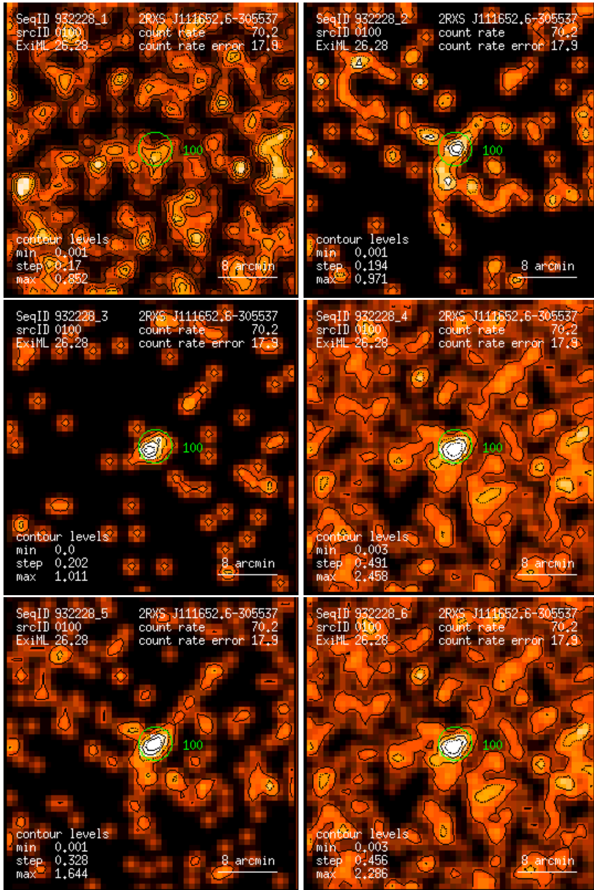
Figure 100: RASS 932228: detection 0100: band rate images, Gaussian filter: (1) PSPC channels 11 – 41, (2) 52 – 90, (3) 91 – 201, (4) 11 – 235, (5) 52 – 201, (6) 11 – 201. Broad band rates in counts/ks. Band rate contour levels in counts/ks/arcmin 2 .
