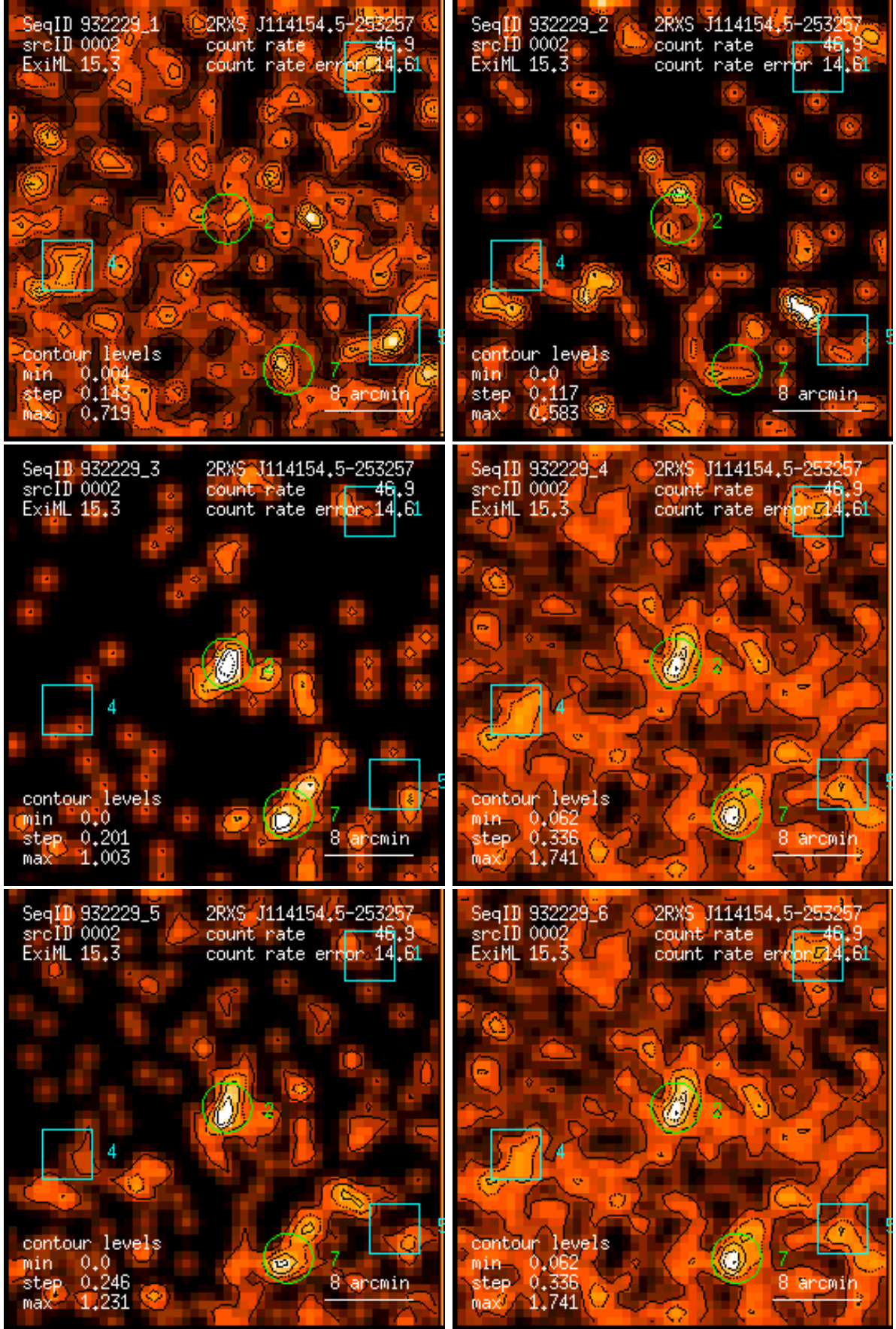
Figure 2: RASS 932229: detection 0002: band rate images, Gaussian filter: (1) PSPC channels 11 – 41, (2) 52 – 90, (3) 91 – 201, (4) 11 – 235, (5) 52 – 201, (6) 11 – 201. Broad band rates in counts/ks. Band rate contour levels in counts/ks/arcmin 2 .
